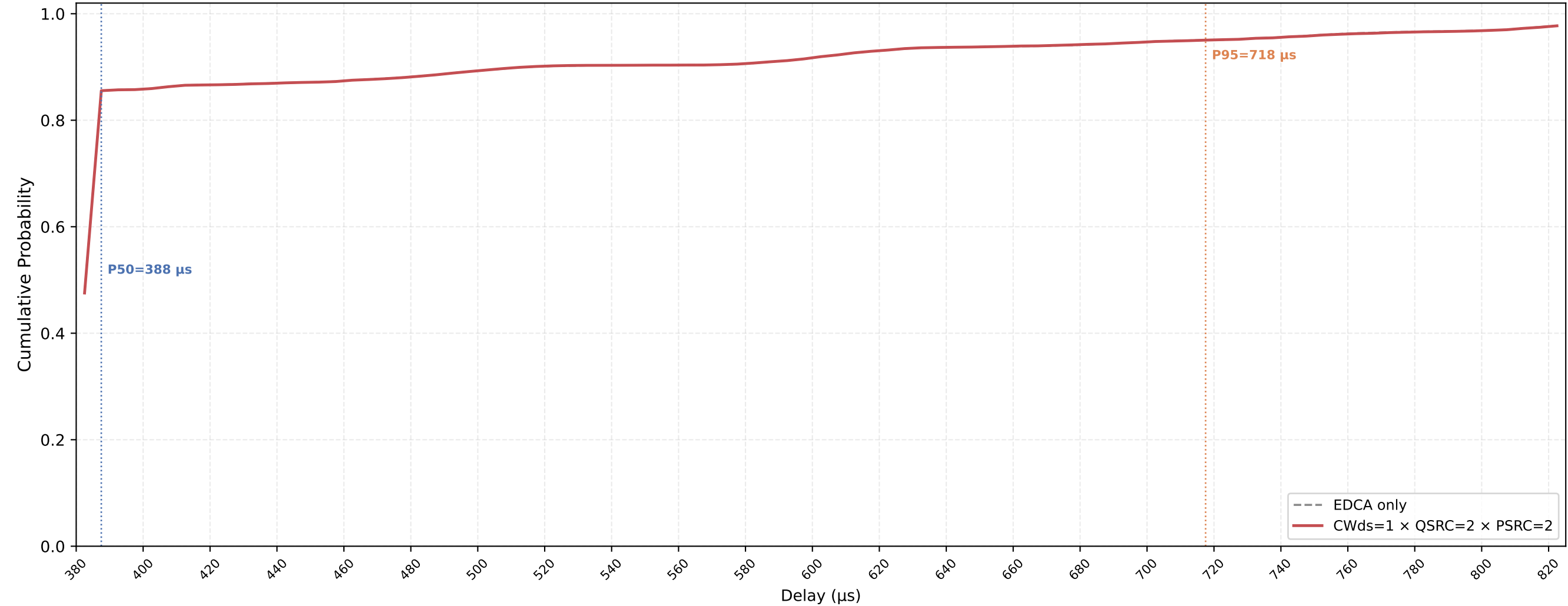
VO (all STAs) Delay CDF — CWds=1 × QSRC=2 × PSRC=2 nSta=30, nPedca=5, 0.1Mbps, avg of 10 runs
