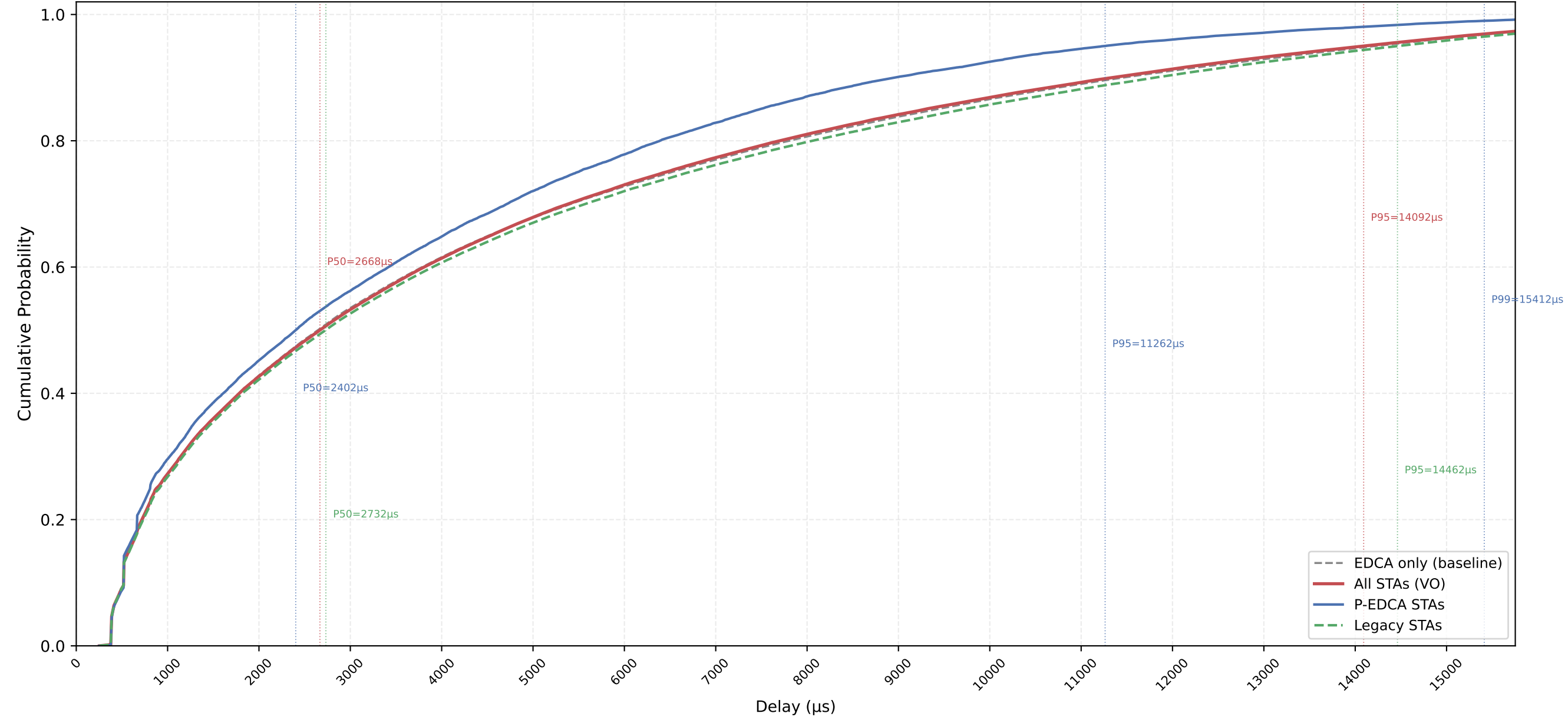
VO Delay CDF — P-EDCA / Legacy / All | CWds=1 × QSRC=2 × PSRC=3 nSta=30, nPedca=5/30, 0.5Mbps, avg of 10 runs
