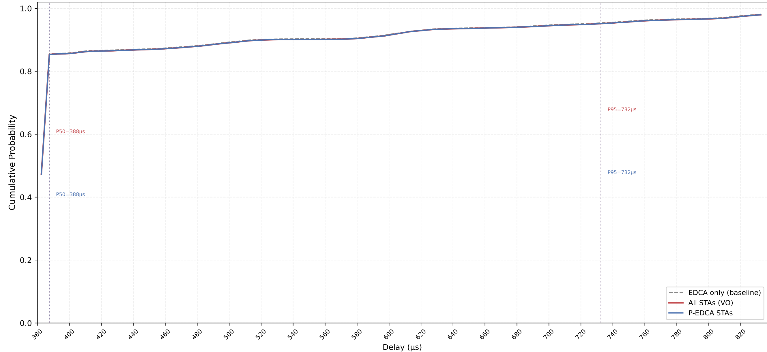
VO Delay CDF — P-EDCA / Legacy / All | CWds=1 × QSRC=3 × PSRC=1 nSta=30, nPedca=30/30, 0.1Mbps, avg of 10 runs
