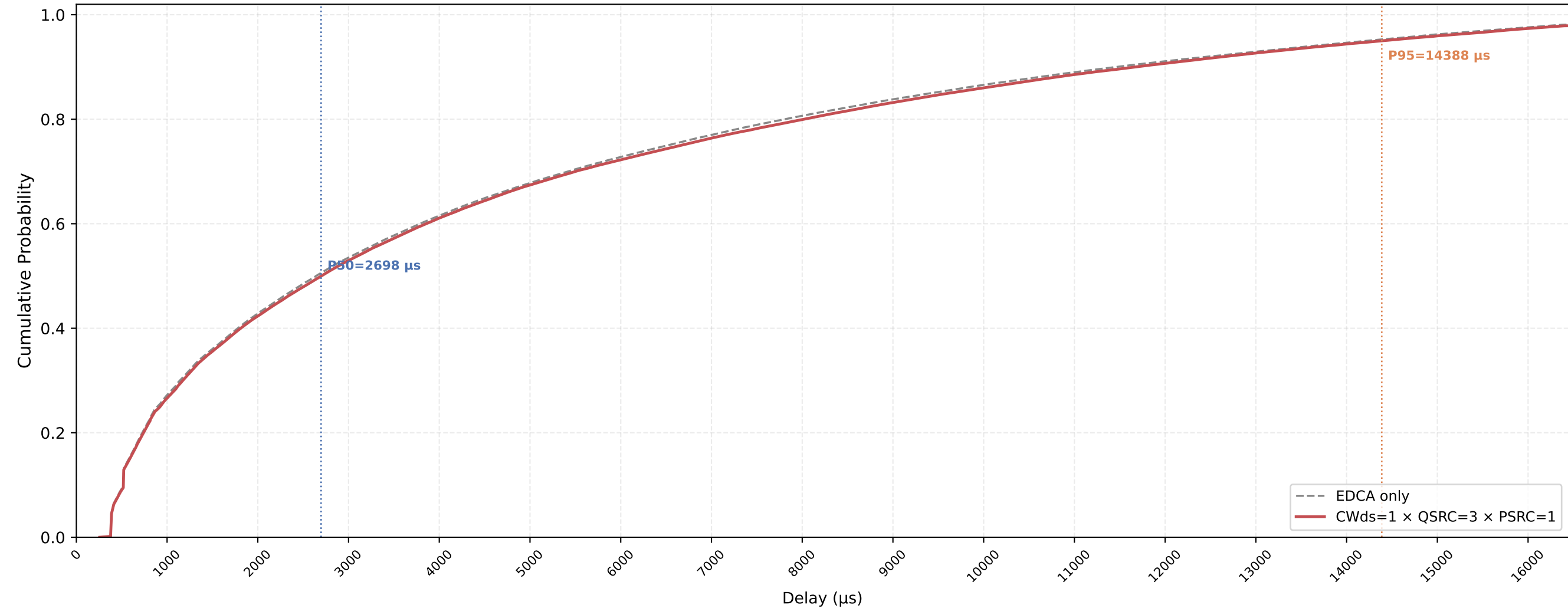
Legacy STA VO Delay CDF — CWds=1 × QSRC=3 × PSRC=1 nSta=30, nPedca=5, 0.5Mbps, avg of 10 runs
