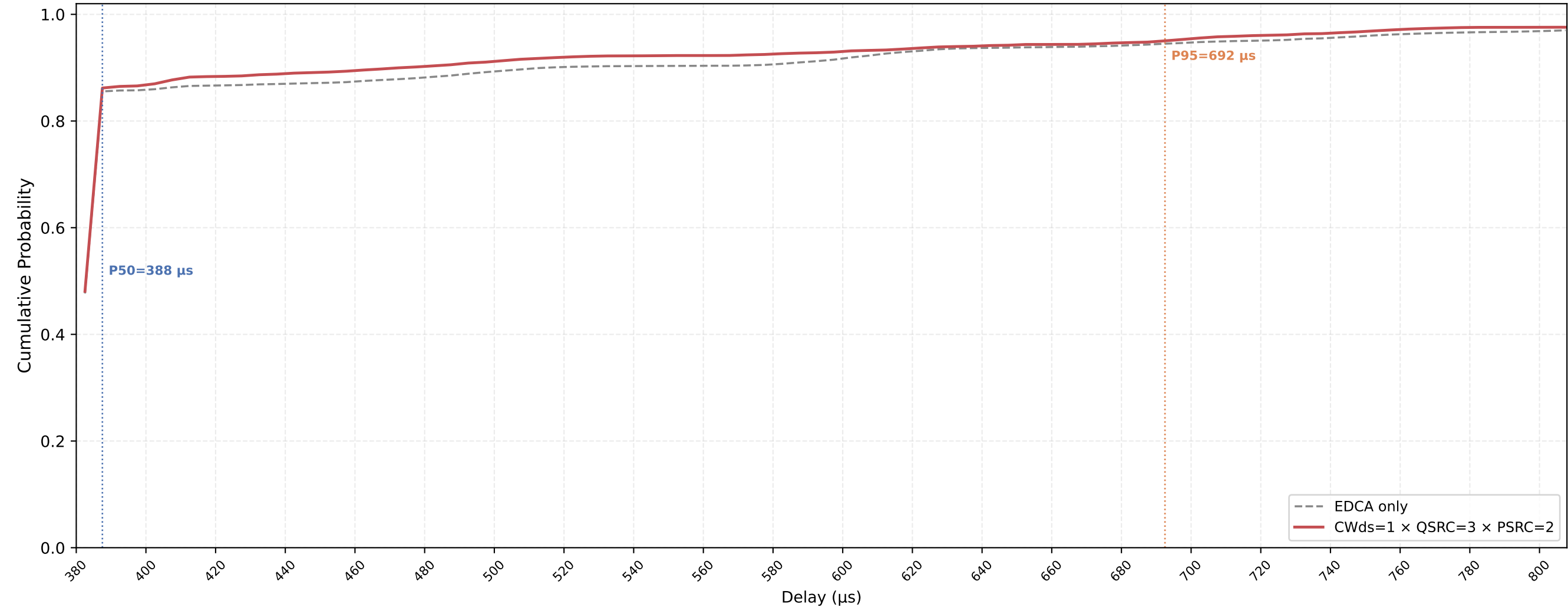
P-EDCA STA VO Delay CDF — CWds=1 × QSRC=3 × PSRC=2 nSta=30, nPedca=15, 0.1Mbps, avg of 10 runs
