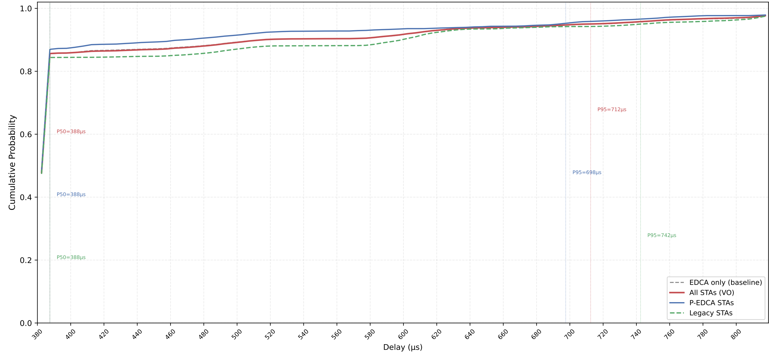
VO Delay CDF — P-EDCA / Legacy / All | CWds=1 × QSRC=3 × PSRC=3 nSta=30, nPedca=15/30, 0.1Mbps, avg of 10 runs
