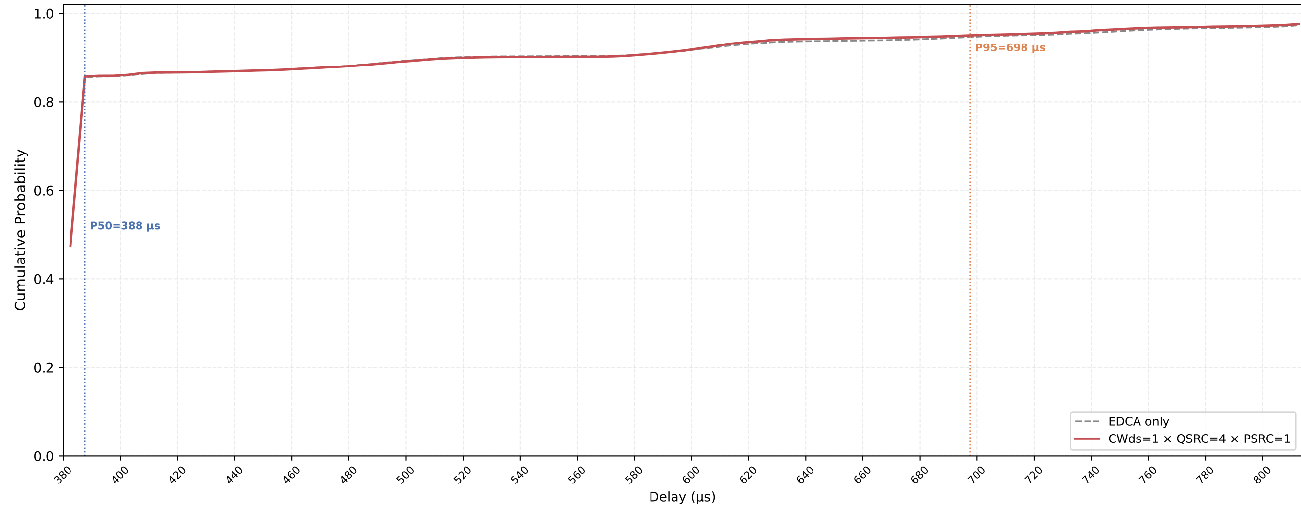
Legacy STA VO Delay CDF — CWds=1 × QSRC=4 × PSRC=1 nSta=30, nPedca=5, 0.1Mbps, avg of 10 runs
