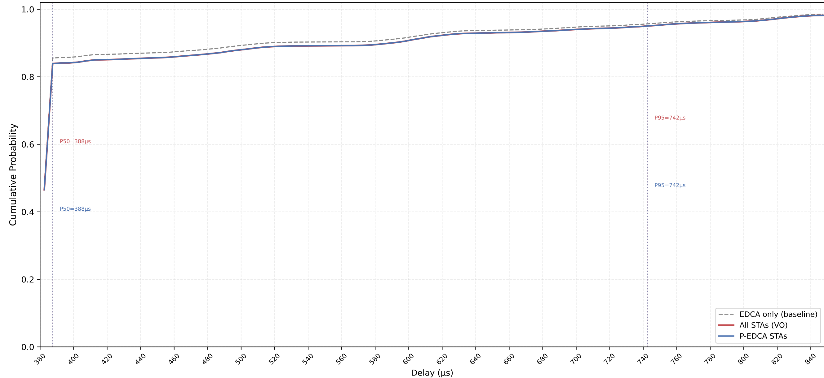
VO Delay CDF — P-EDCA / Legacy / All | CWds=1 × QSRC=4 × PSRC=2 nSta=30, nPedca=30/30, 0.1Mbps, avg of 10 runs
