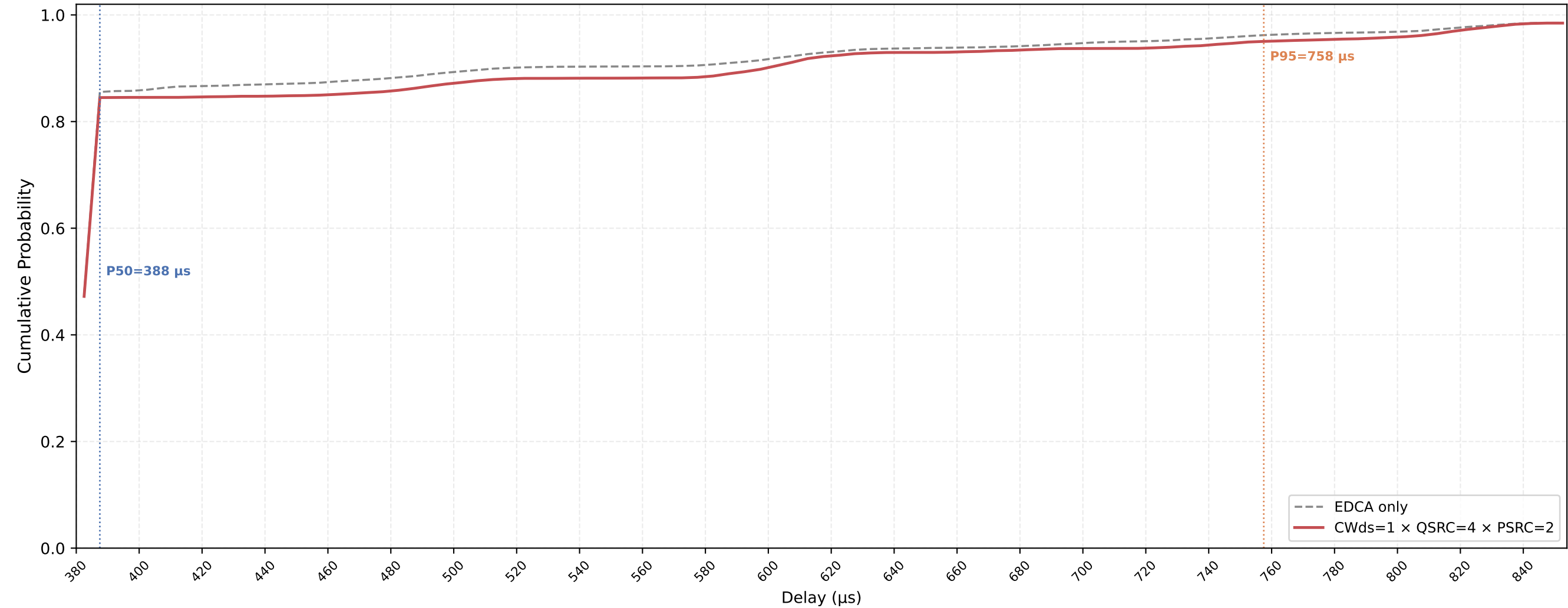
Legacy STA VO Delay CDF — CWds=1 × QSRC=4 × PSRC=2 nSta=30, nPedca=15, 0.1Mbps, avg of 10 runs
