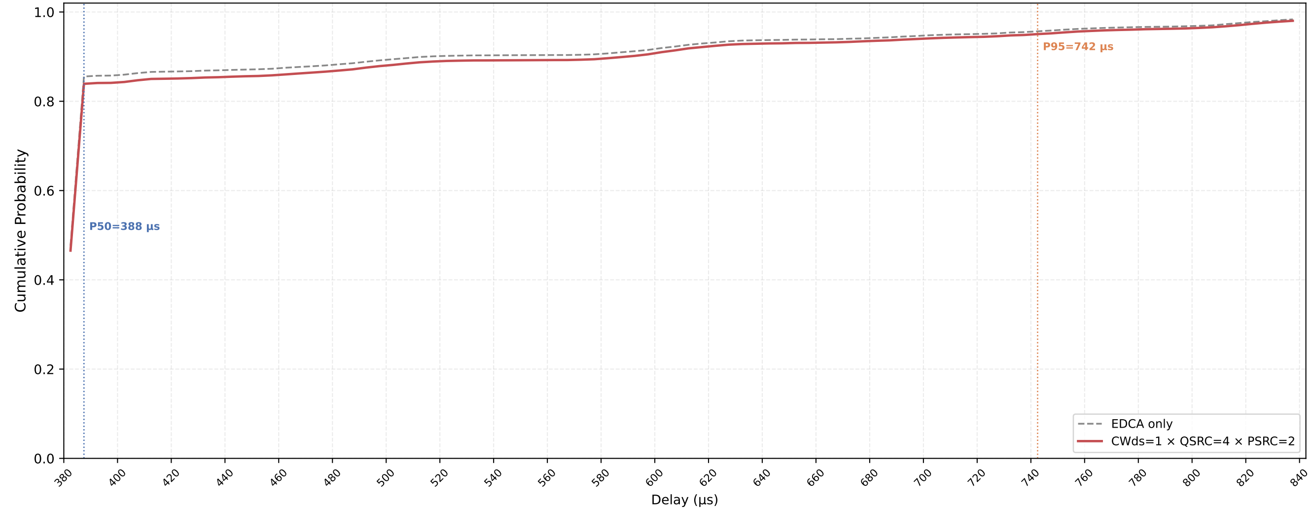
P-EDCA STA VO Delay CDF — CWds=1 × QSRC=4 × PSRC=2 nSta=30, nPedca=30, 0.1Mbps, avg of 10 runs
