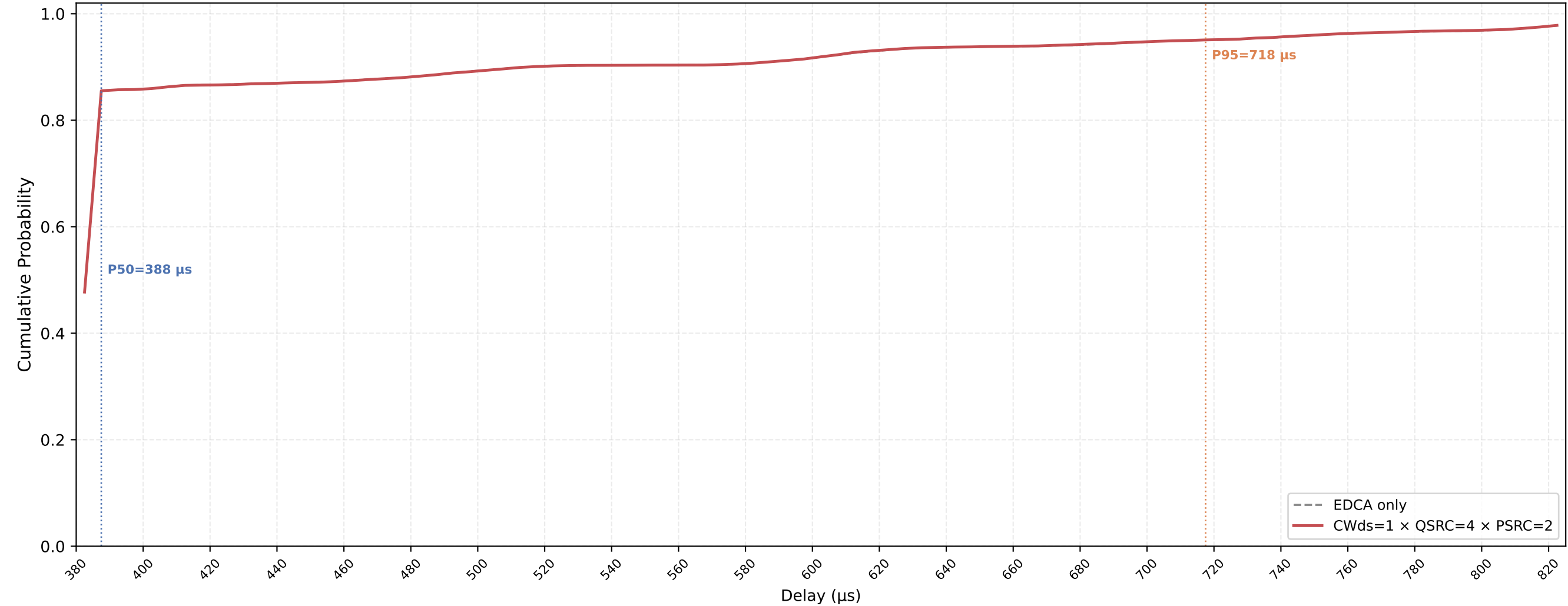
VO (all STAs) Delay CDF — CWds=1 × QSRC=4 × PSRC=2 nSta=30, nPedca=5, 0.1Mbps, avg of 10 runs
