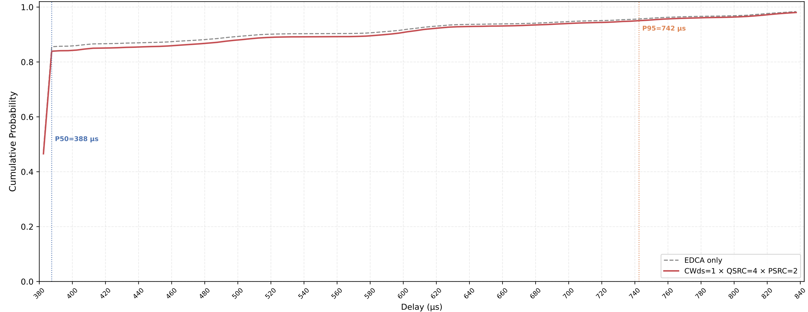
VO (all STAs) Delay CDF — CWds=1 × QSRC=4 × PSRC=2 nSta=30, nPedca=30, 0.1Mbps, avg of 10 runs
