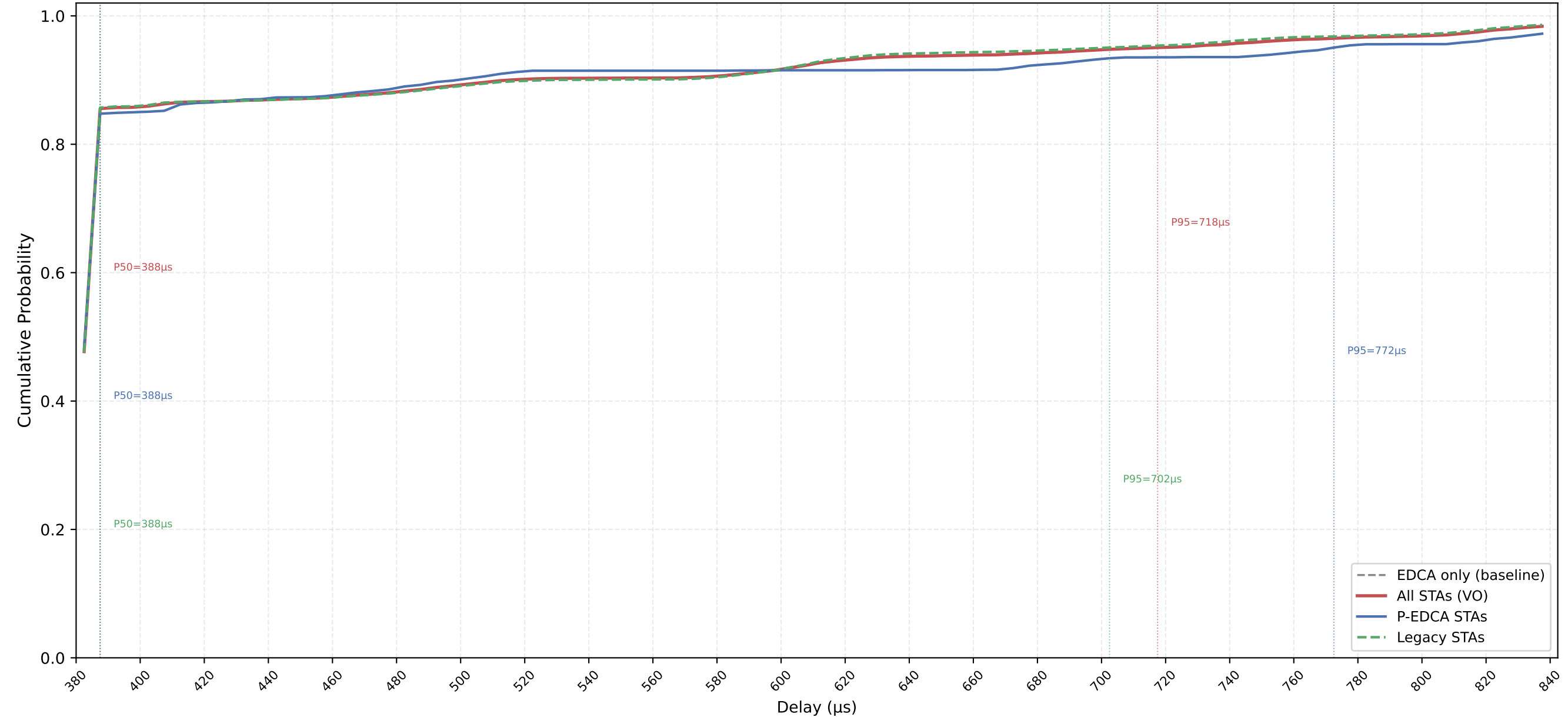
VO Delay CDF — P-EDCA / Legacy / All | CWds=1 × QSRC=4 × PSRC=3 nSta=30, nPedca=5/30, 0.1Mbps, avg of 10 runs
