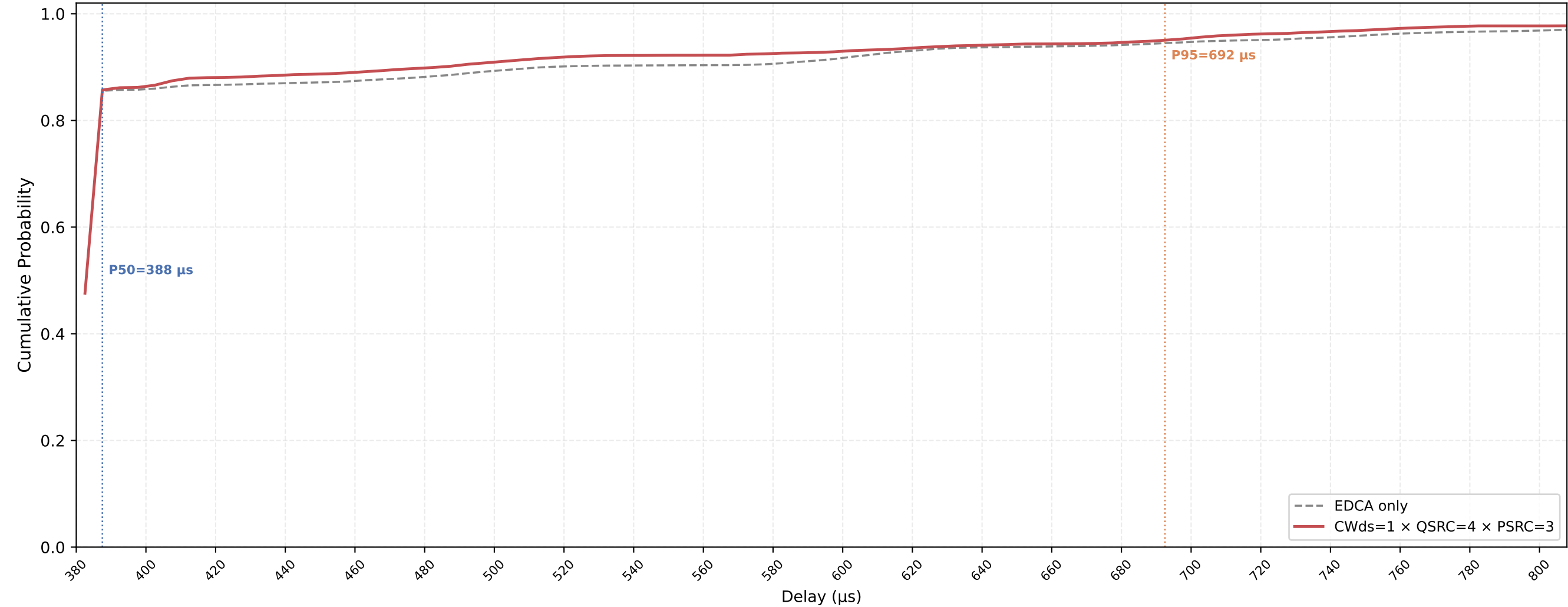
P-EDCA STA VO Delay CDF — CWds=1 × QSRC=4 × PSRC=3 nSta=30, nPedca=15, 0.1Mbps, avg of 10 runs
