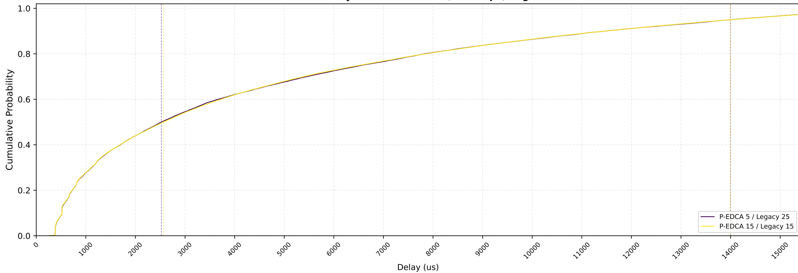
P-EDCA STAs Delay CDF — nSta=30, 0.5Mbps, avg of 10 runs
