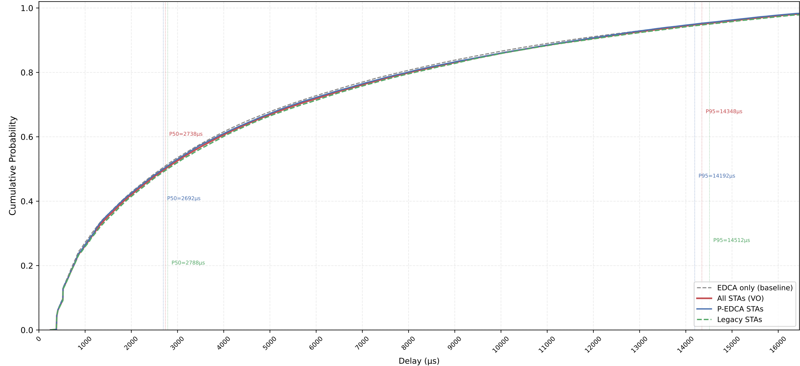
VO Delay CDF — P-EDCA / Legacy / All | CWds=1 × QSRC=5 × PSRC=1 nSta=30, nPedca=15/30, 0.5Mbps, avg of 10 runs
