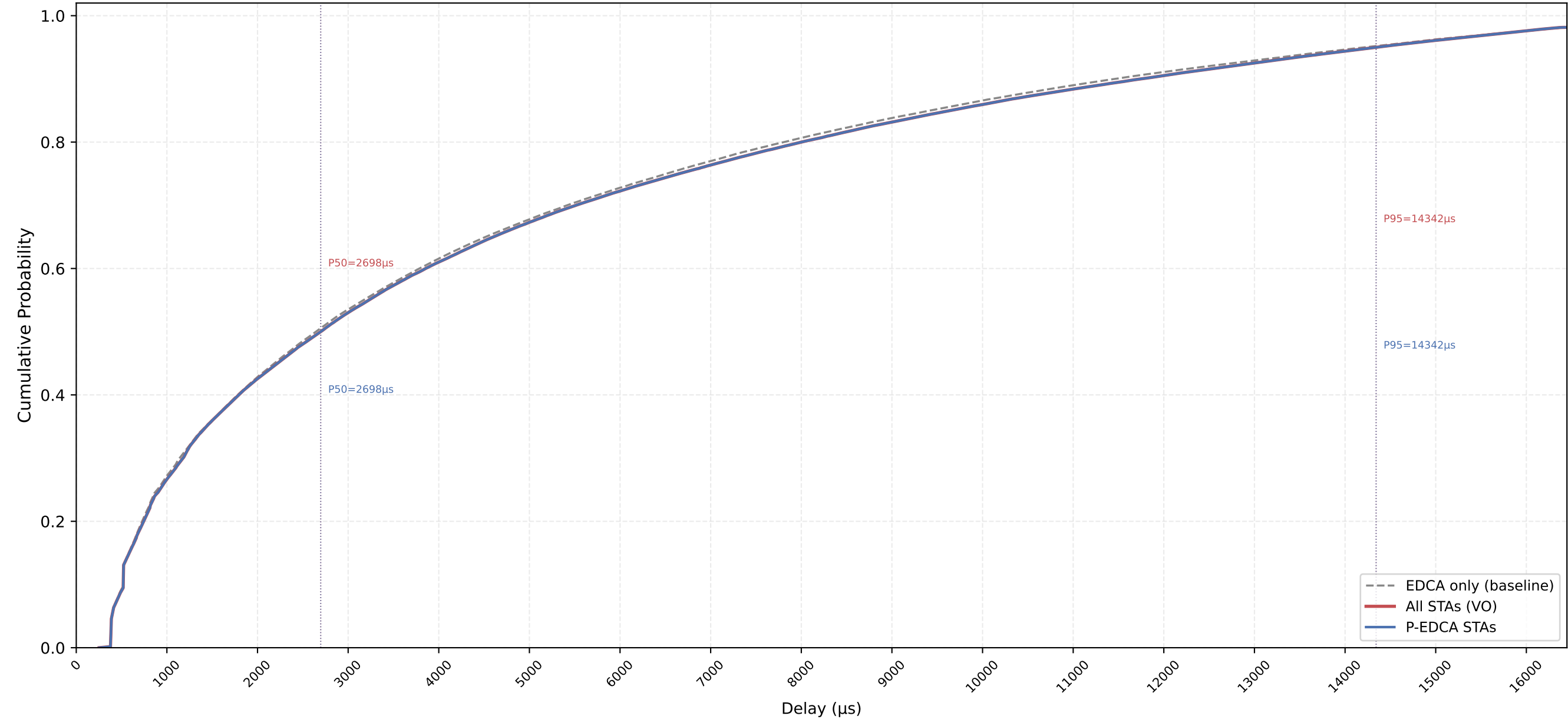
VO Delay CDF — P-EDCA / Legacy / All | CWds=1 × QSRC=5 × PSRC=1 nSta=30, nPedca=30/30, 0.5Mbps, avg of 10 runs
