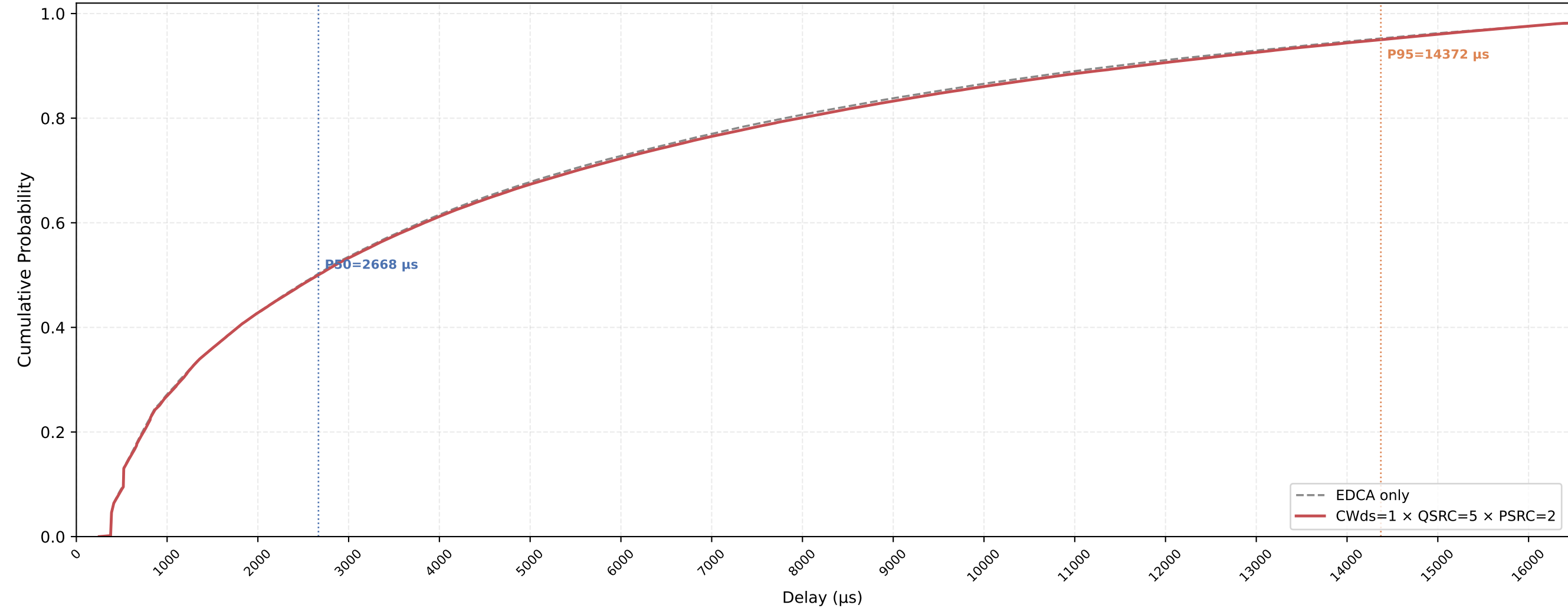
VO (all STAs) Delay CDF — CWds=1 × QSRC=5 × PSRC=2 nSta=30, nPedca=15, 0.5Mbps, avg of 10 runs
