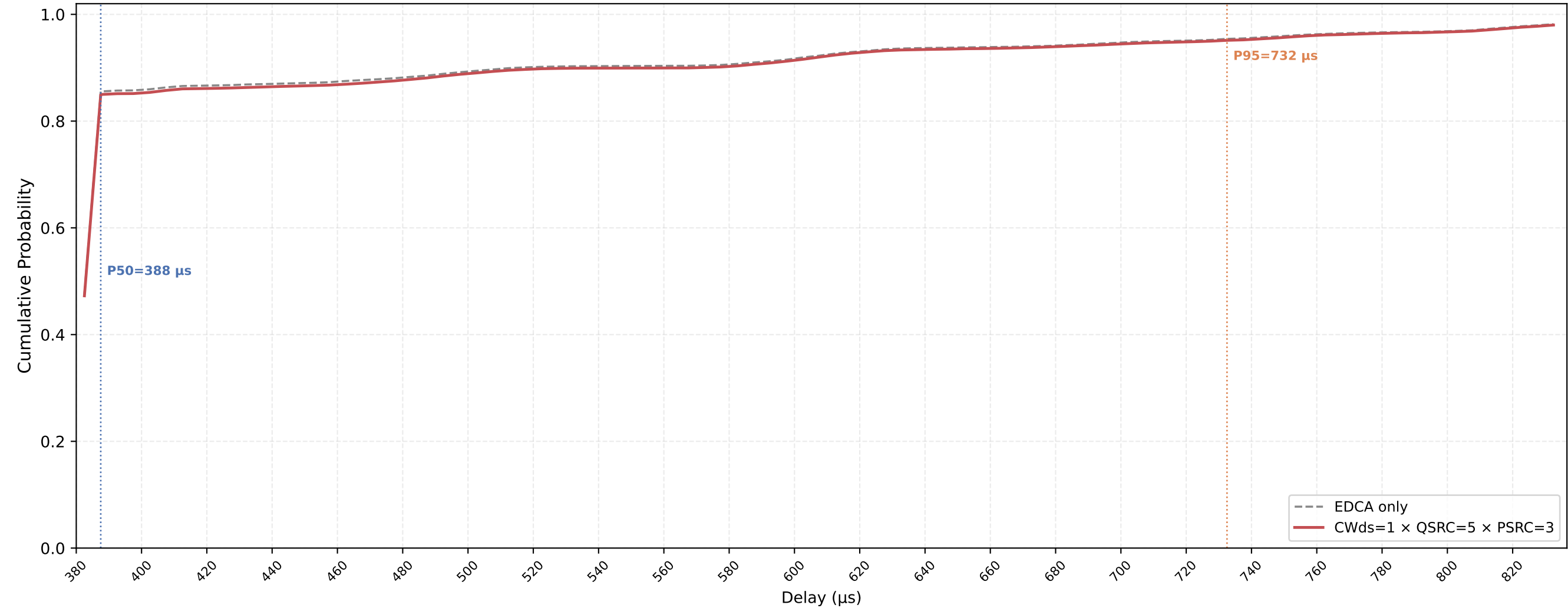
VO (all STAs) Delay CDF — CWds=1 × QSRC=5 × PSRC=3 nSta=30, nPedca=30, 0.1Mbps, avg of 10 runs
