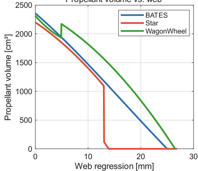
Propellant volume vs. web
