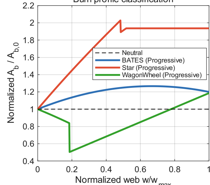
Burn profile classification
