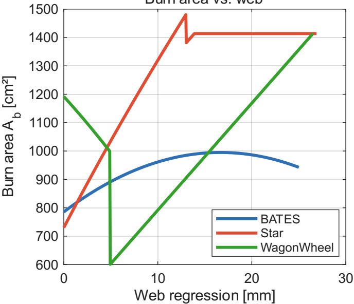
Burn area vs. web
