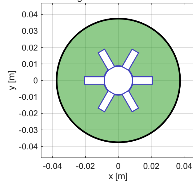
WagonWheel — OD 75mm
