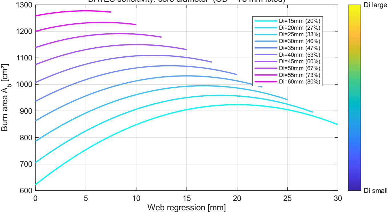
BATES sensitivity: core diameter (OD = 75 mm fixed)
