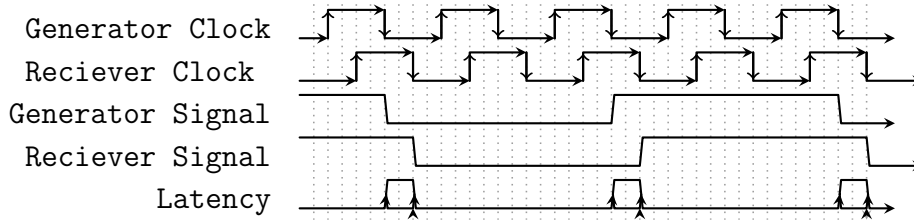
Figure 7.3: Test Harness Capture
