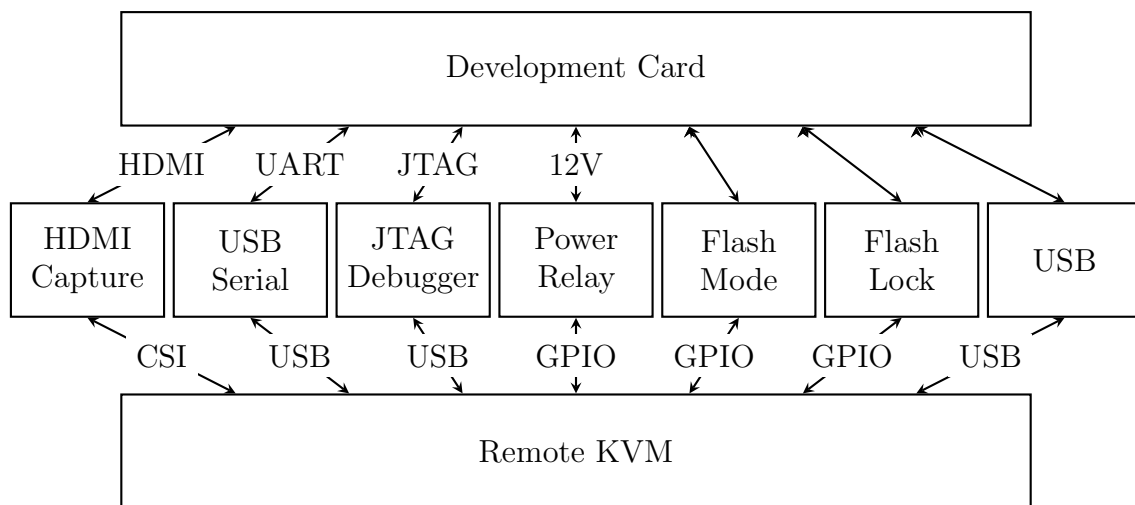
Figure 7.5: Development Hardware
