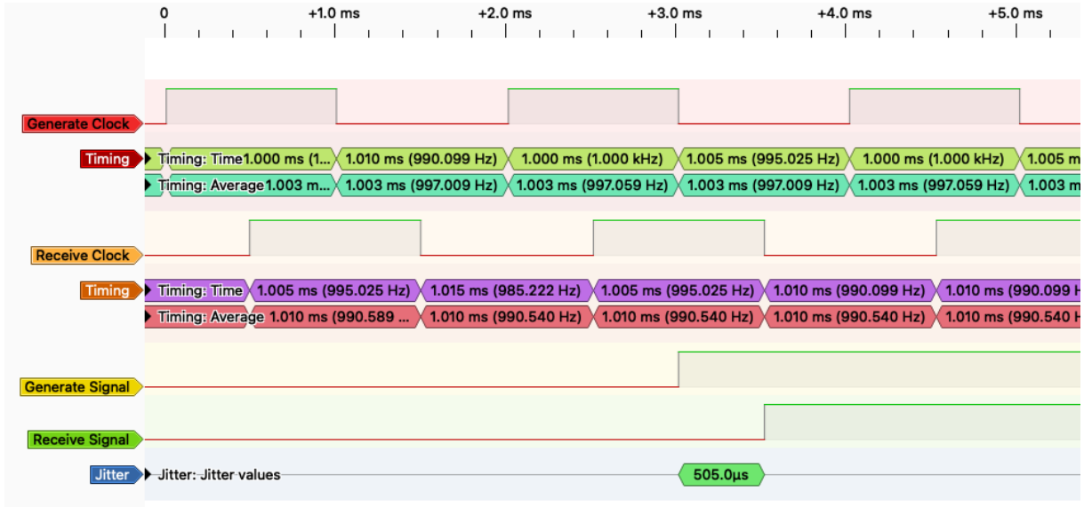
Figure 7.4: Test Harness PluseView Capture
