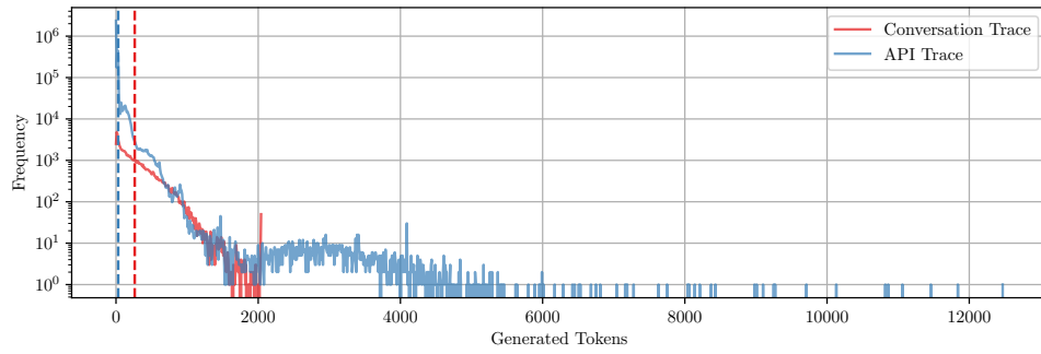
Figure 5.9: Decode Tokens
