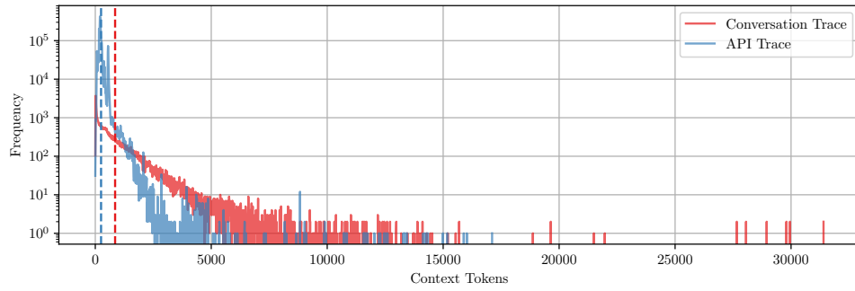
Figure 5.8: Context Tokens
