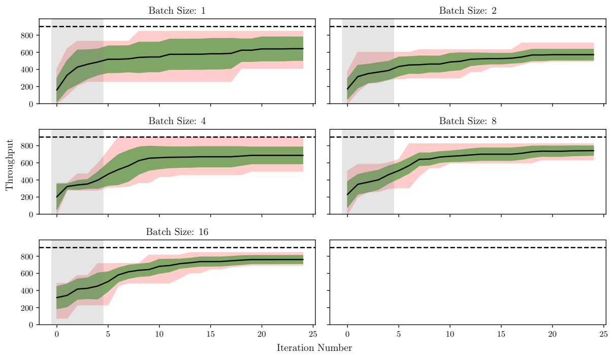
Figure 5.5: Batch Size Analysis
