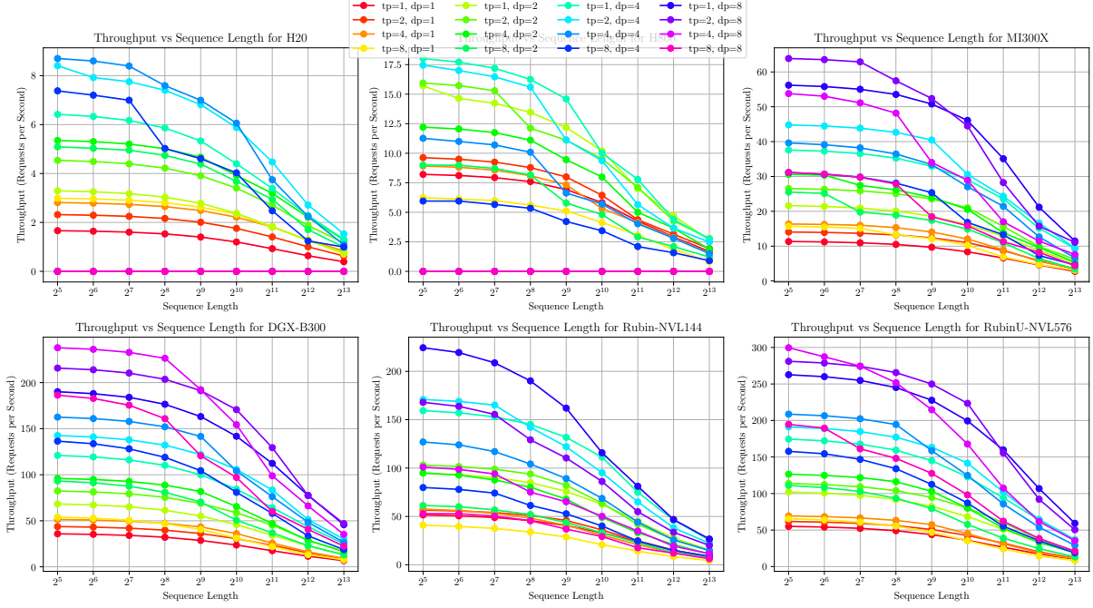
Figure 4.6: Selection of GPUs benchmarked over the decode stage, with a variety of parallelism configurations using the Shallowsim simulator. All configurations use a static number of GPUs (64).
