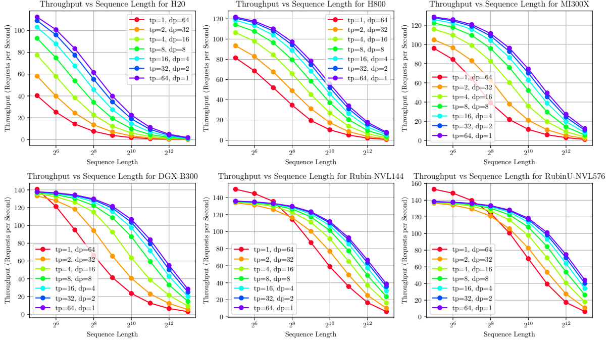
Figure 4.5: Selection of GPUs benchmarked over the prefill stage, with a variety of parallelism configurations using the Shallowsim simulator. All configurations use a static number of GPUs (64).
