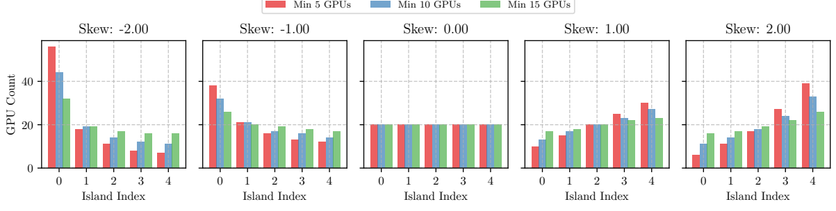
Figure 4.10: Graph displaying the effect of changing the S_{\text{skew}} value where G_{\text{total}} = 100 and N_{\text{target}} = 5 . Instances with high skew values (absolute), display higher island size variance.
