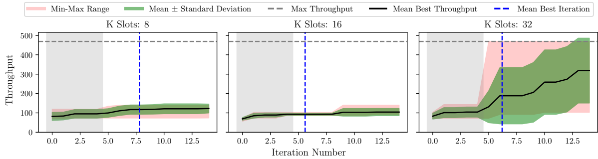
Figure 5.10: Throughput per iteration number for different K slots (Direct SAASBO). Experiment Parameters: batch size = 4, iterations = 10, trials = 5
