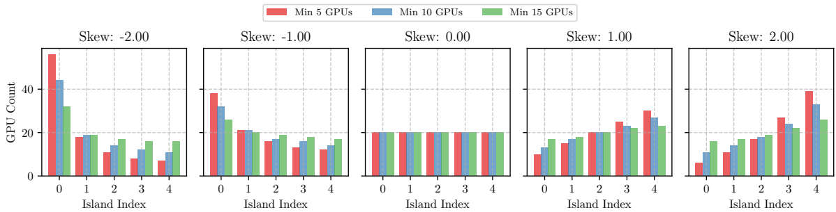
Figure 4.10: Graph displaying the effect of changing the S_{\text{skew}} value where G_{\text{total}} = 100 and N_{\text{target}} = 5 . Instances with high skew values (absolute), display higher island size variance.
