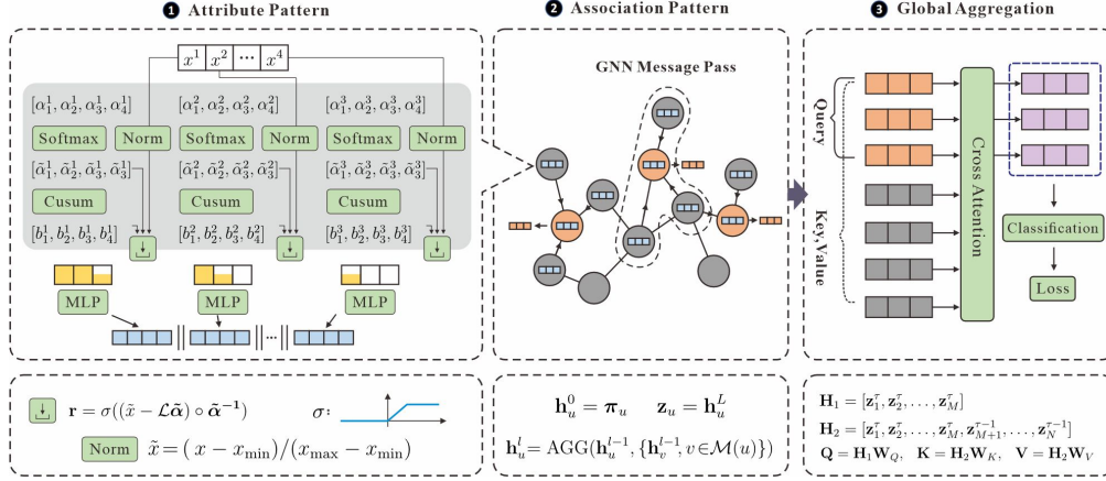
Figure 1: The GAAP framework. DyBEM creates binned attribute patterns, GraphSAGE (Eq. 1) extracts association patterns, and global cross-attention captures pattern correlations. RP-GAAP adds rarity weights (Eq. 2) to the loss without modifying this architecture. Figure adapted from [2].
