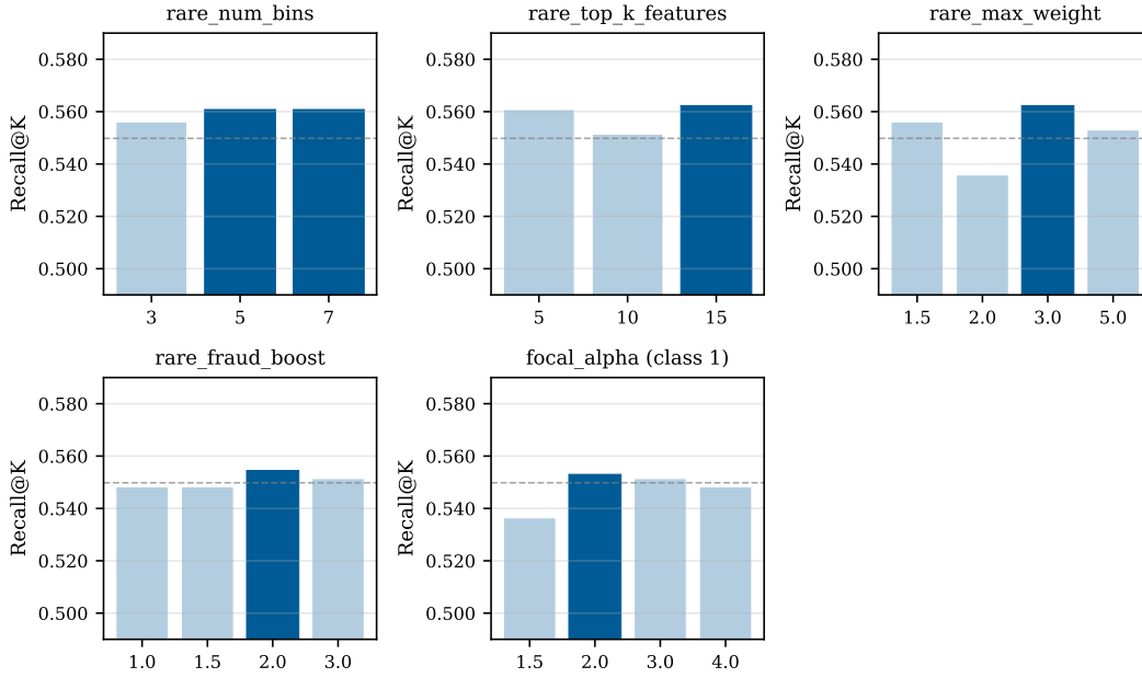
Figure 3: Hyperparameter sensitivity on Tolokers. Each subplot shows Recall@K as a function of a single parameter, with all others held at default values. The dashed horizontal line indicates the GAAP baseline Recall@K.
