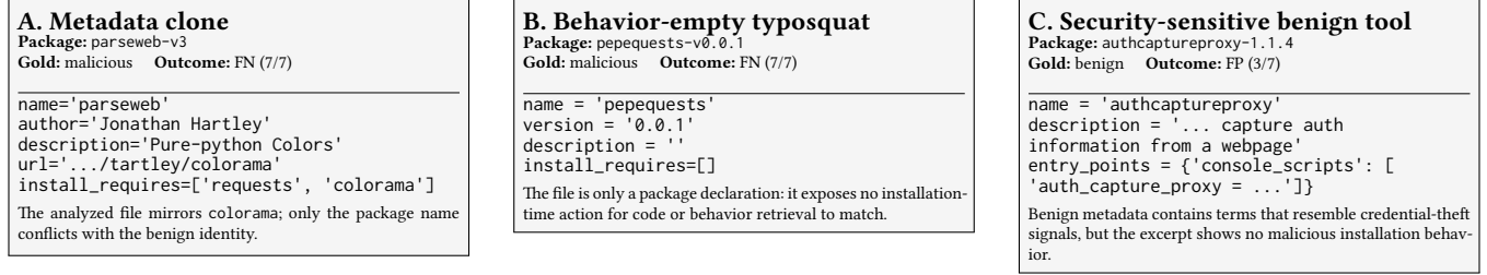
Figure 2: Concrete error examples from the held-out setup.py files. FN and FP denote false negative and false positive, respectively; the parenthesized count is the number of Llama configurations making that error. Excerpts are shortened only for presentation.
