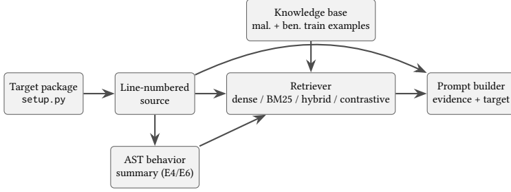
Figure 1: Overview of the evaluated pipelines. All stages are shared across methods except query construction and retrieval (E4/E6 additionally build an AST behavior summary as the query).
