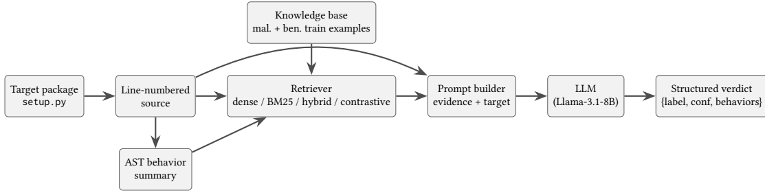
Figure 1: Overview of the evaluated pipelines. All stages are shared across methods except query construction and retrieval (the behavior-based methods additionally build an AST behavior summary as the query).
