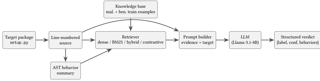
Figure 1: Overview of the seven controlled Llama retrieval configurations. All stages are shared across methods except query construction and retrieval (the behavior-based methods additionally build an AST behavior summary as the query).
