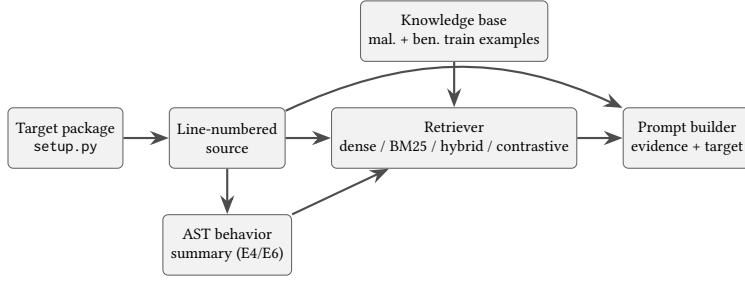
Figure 2: Overview of the evaluated pipelines. All stages are shared across methods except query construction and retrieval (E4/E6 additionally build an AST behavior summary as the query).
