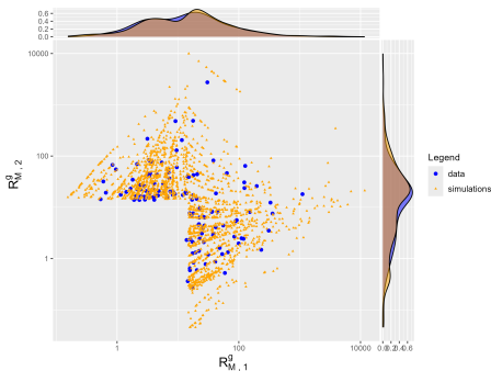
Figure 13: Simulation of radial components
