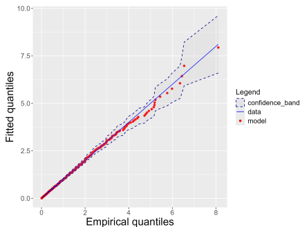
Figure 10: EGPD fitting: a)Hs, b)Surge
