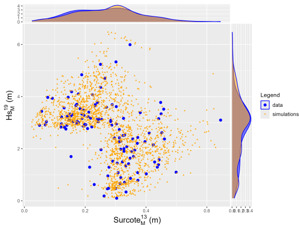
Figure 31: Distribution of (\text{Surge}(t), H_s(s))
