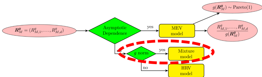
Figure 12: Model used in case of asymptotic independence
