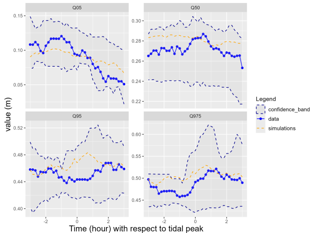
Figure 25: QQ results for the surge
