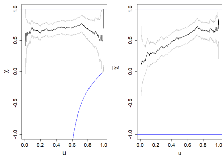
Figure 16: Extremal correlation coefficients for H_s at time t = 1, s = 37
