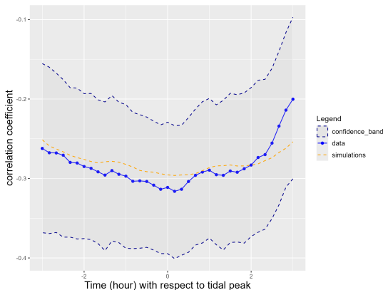
Figure 30: Correlation coefficients for each value of t
