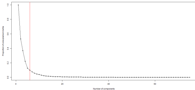
Figure 17: Evolution of unexplained inertia
