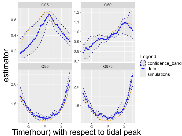
Figure 21: Evolution of several quantiles for \Omega_{M,1}
