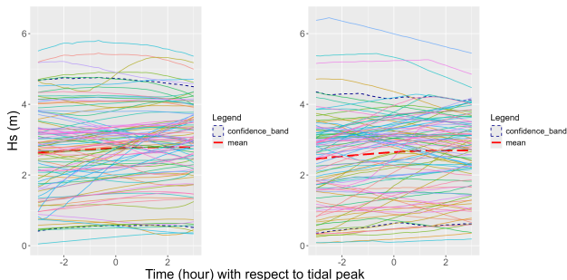
Figure 20: Simulated (left panel) and observed (right panel) extreme time series for Hs
