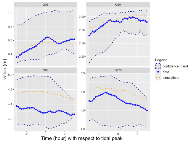
Figure 24: QQ results for Hs
