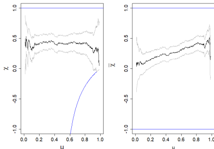
Figure 34: Extremal correlation coefficients for wind speed at time t = 1, s = 37
