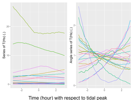
Figure 9: Sampling of 20 Hs time series with decomposition: Z_{M,2} (left panel), \Theta_{M,2} (right panel)
