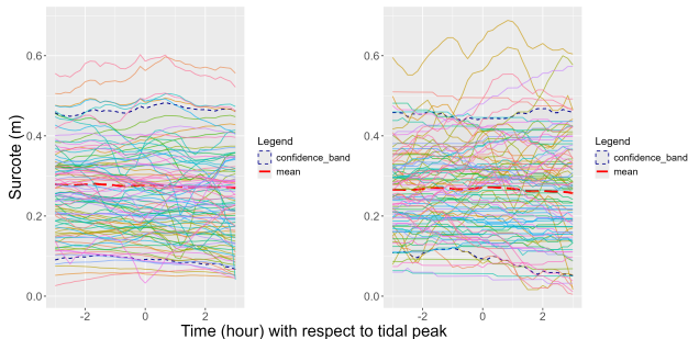
Figure 19: Simulated (left panel) and observed (right panel) extreme time series for the surge
