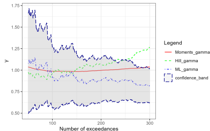
Figure 6: Estimation of \gamma for: \ell(\mathbf{Z}_{M,1}) ; \ell(\mathbf{Z}_{M,2}) (solid line: moments estimator, dotted line: Hill estimator, dashed line: MLE estimator)
