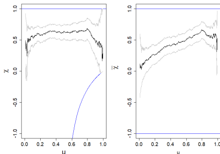
Figure 33: Extremal correlation coefficients for wind speed at time t = 1, s = 19
