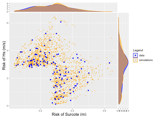
Figure 23: Distribution of risk functions
