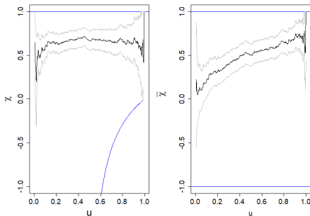
Figure 15: Extremal correlation coefficients for the surge at time t = 1, s = 37
