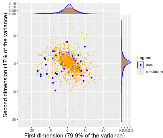
Figure 27: PCA coordinates for extreme Hs time series
