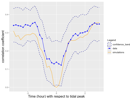
Figure 29: Correlation coefficients for each value of t
