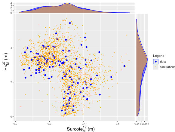
Figure 32: Distribution of (\text{Surge}(t), Hs(s))
