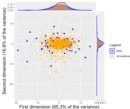
Figure 26: PCA coordinates for extreme surge time series
