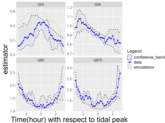
Figure 22: Evolution of several quantiles for \Omega_{M,2}
