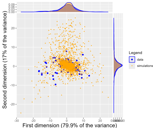
Figure 30: PCA coordinates for extreme Hs time series with logistic model
