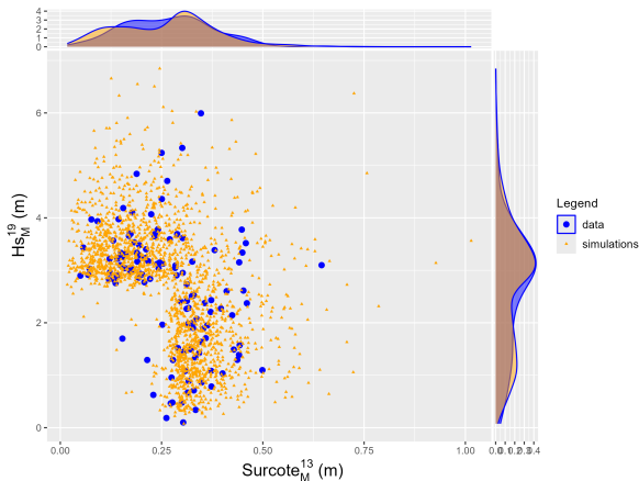
Figure 33: Distribution of (\text{Surge}(t), \text{Hs}(s))
