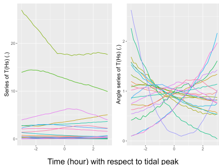
Figure 9: Sampling of 20 Hs time series with decomposition: \mathbf{Z}_{M,2} (left panel), \Theta_{M,2} (right panel)
