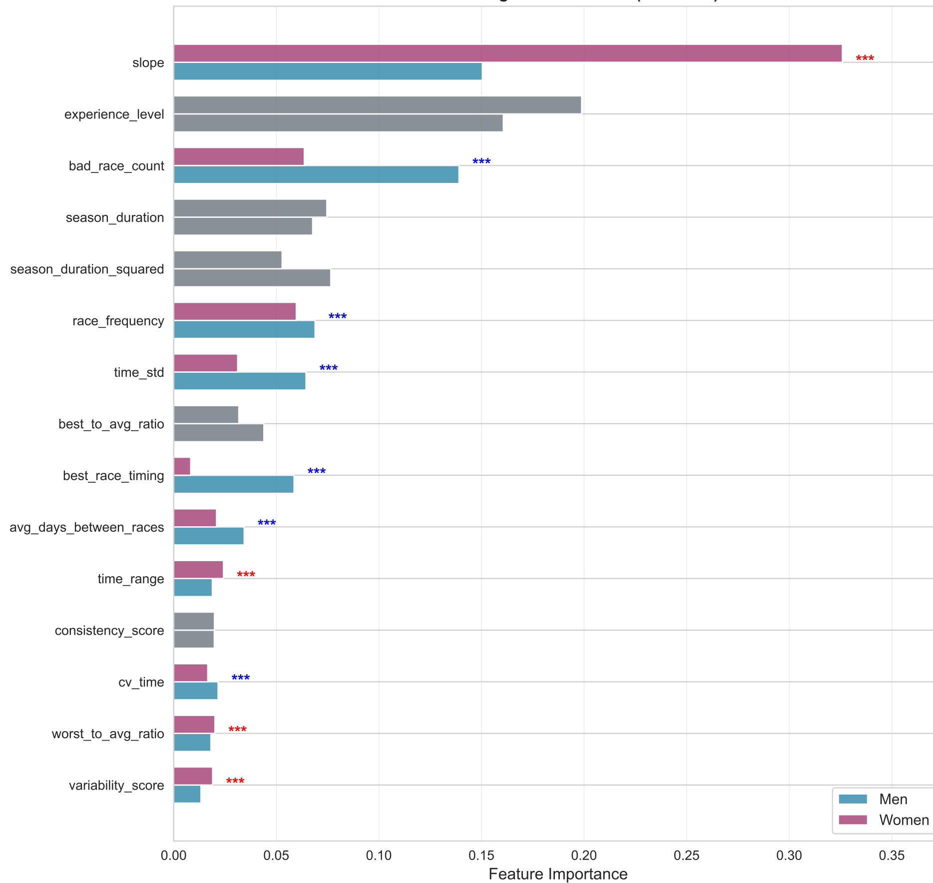
Random Forest Feature Importance Comparison: Men vs Women (Colored = Bonferroni Significant Between Genders, ***p<Bonferroni threshold) Bonferroni Significant: 17 total (10 shown)
