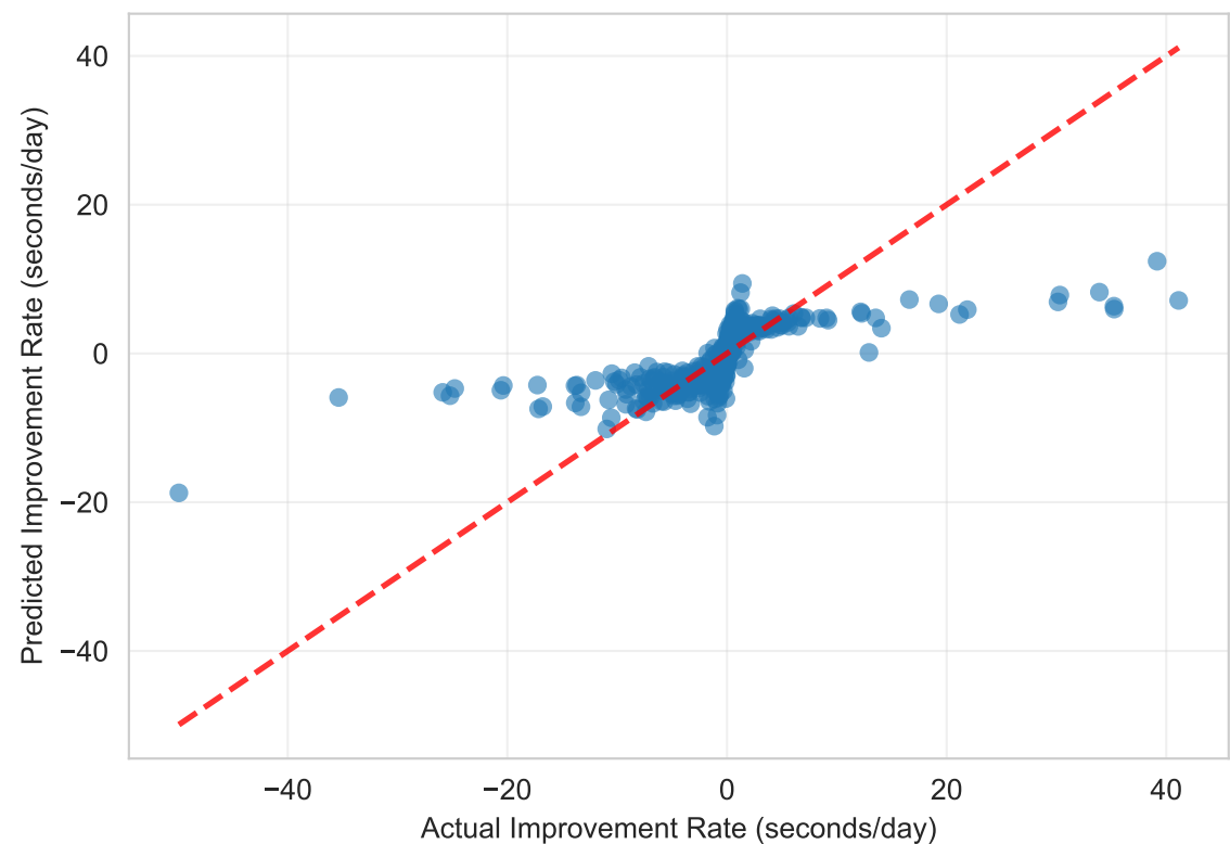
Random Forest R^2 = 0.892 (95% CI: [0.832, 0.946]) n=792
