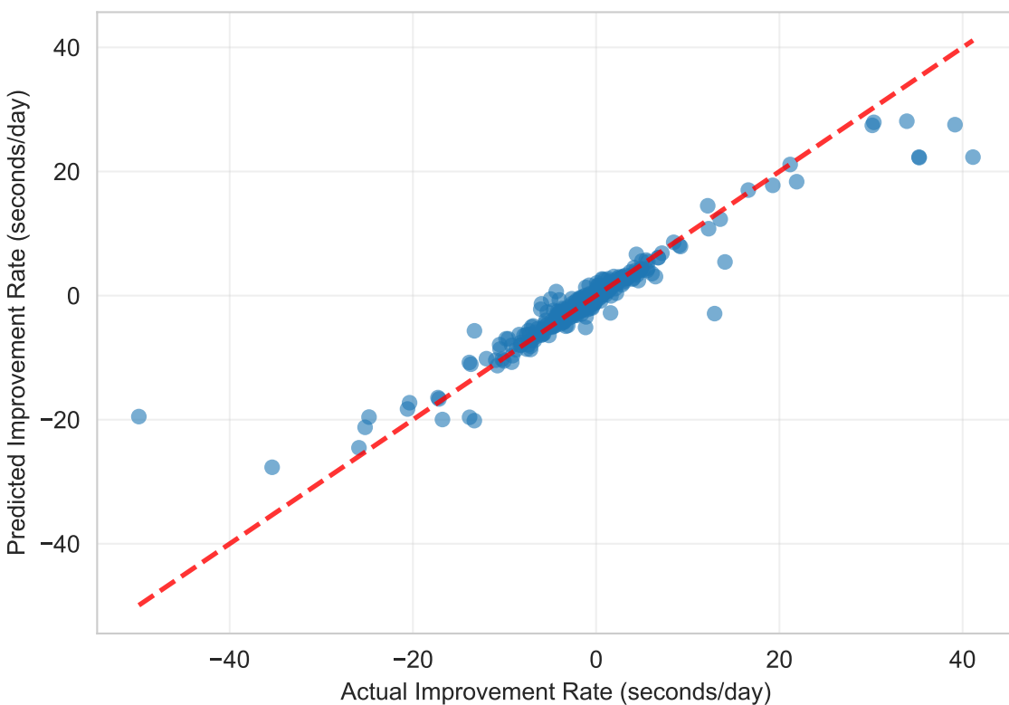
Gradient Boosting R^2 = 0.883 (95% CI: [0.822, 0.939]) n=792
