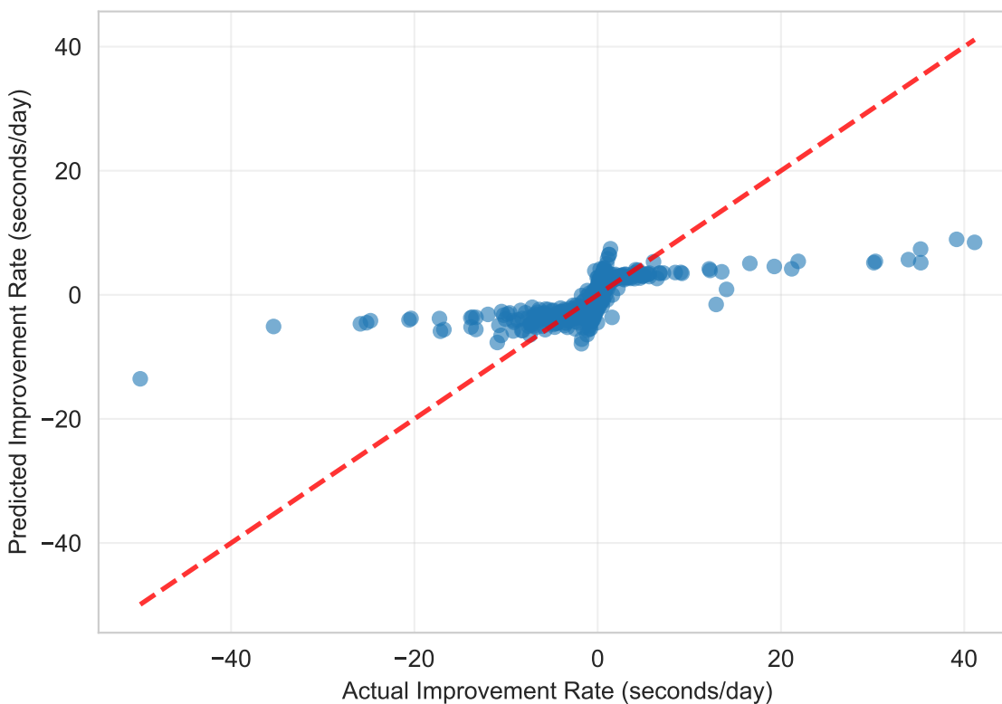
SVR R^2 = 0.498 (95% CI: [0.378, 0.656]) n=792
