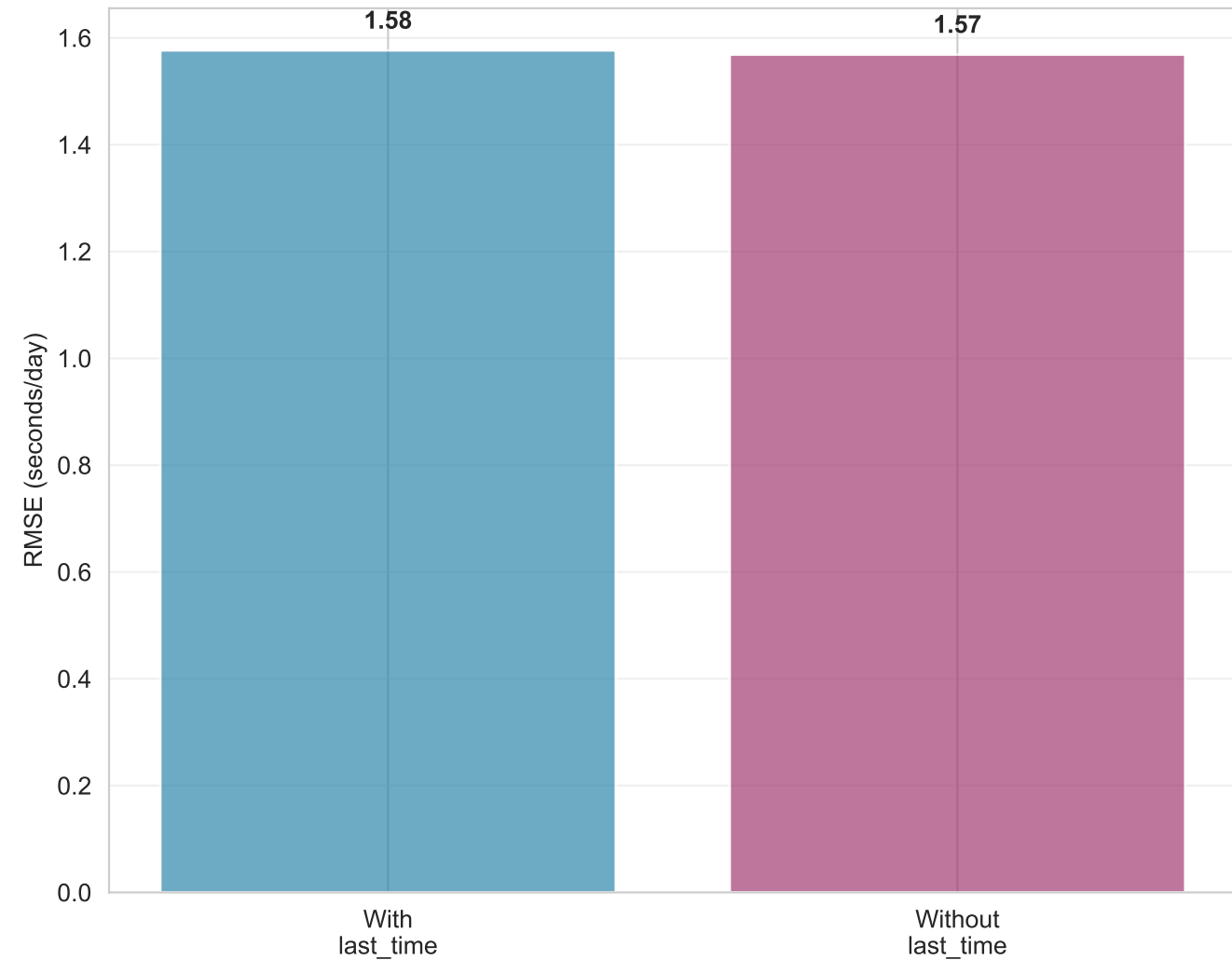
RMSE: With vs Without last_time Feature (Lower is Better)
