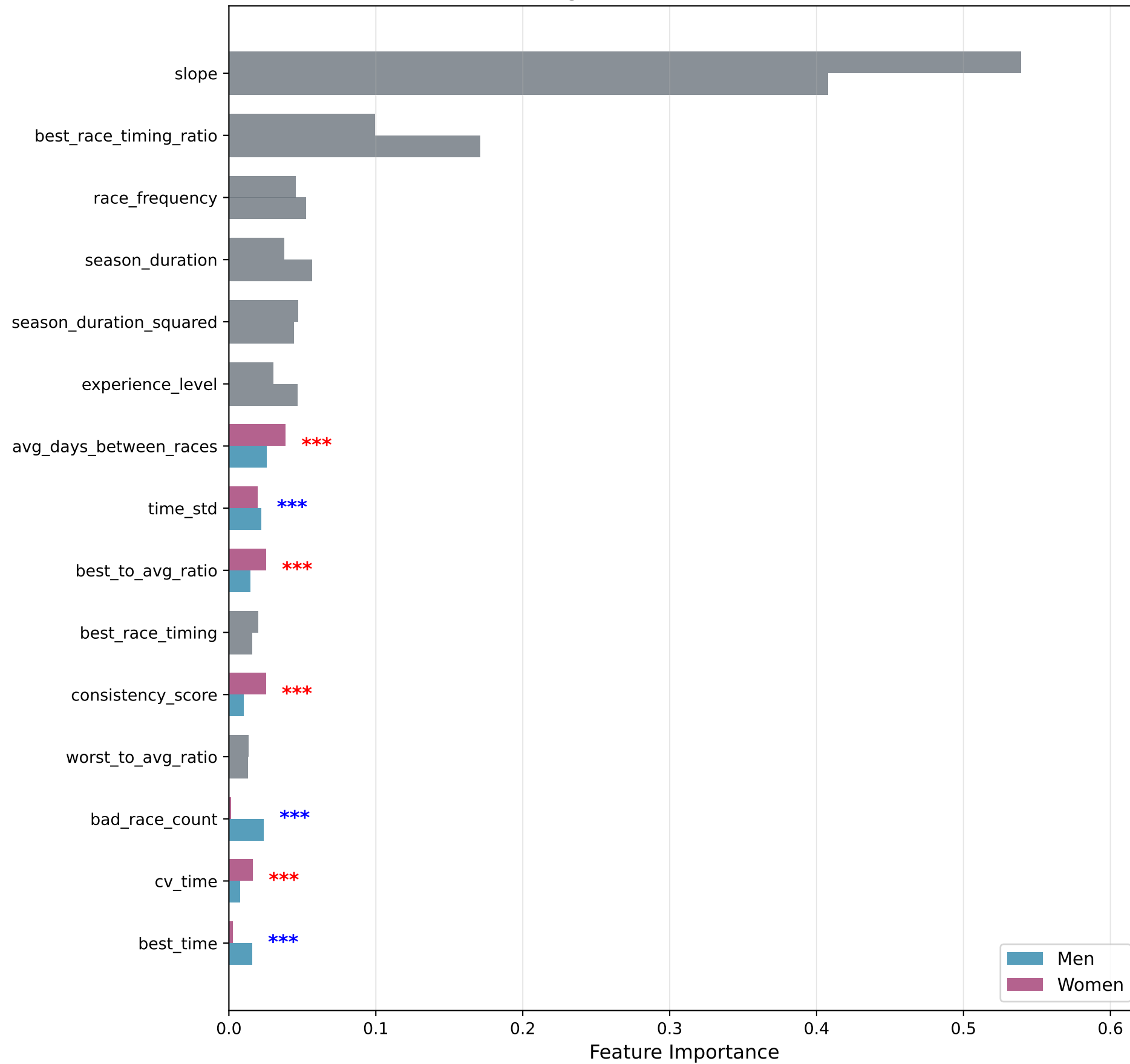
Random Forest Feature Importance Comparison: Men vs Women (Colored = Bonferroni Significant Between Genders, ***p<Bonferroni threshold) Bonferroni Significant: 16 total (7 shown) (RQ2)
