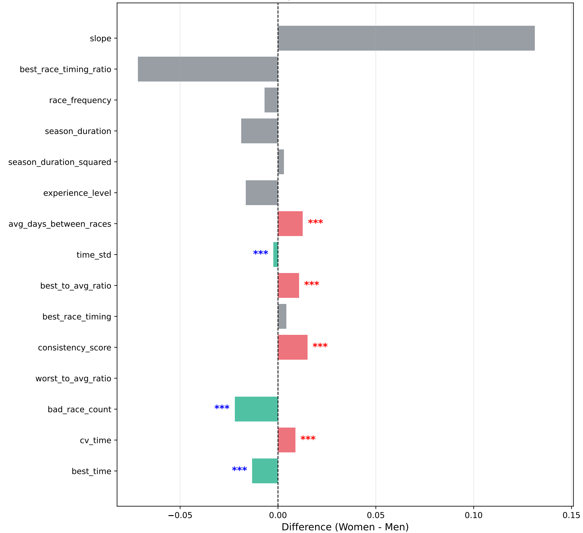
Random Forest Feature Importance Differences (Red/Green = Bonferroni Significant Between Genders, Gray = Not Significant) Bonferroni Significant: 16 total (7 shown) (RQ2)
