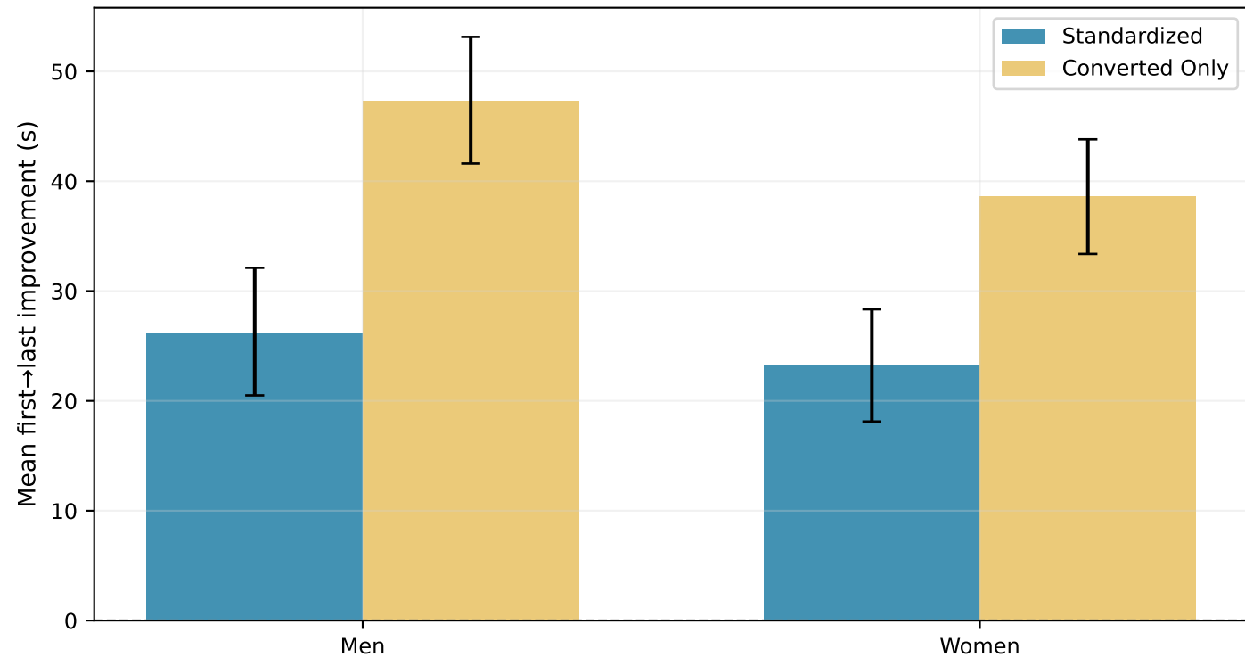
Weather inflation of apparent improvement (Converted Only vs Standardized)
