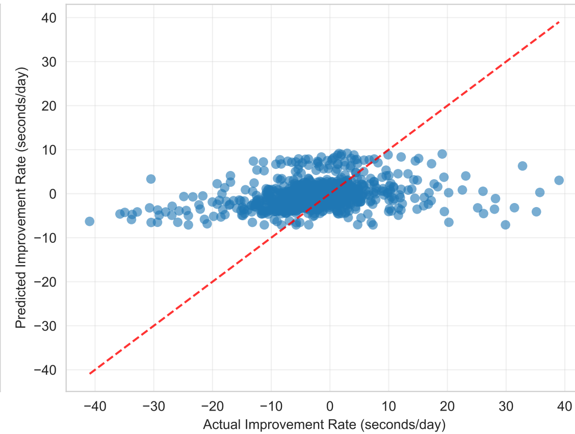
SVR R^2 = 0.0401
