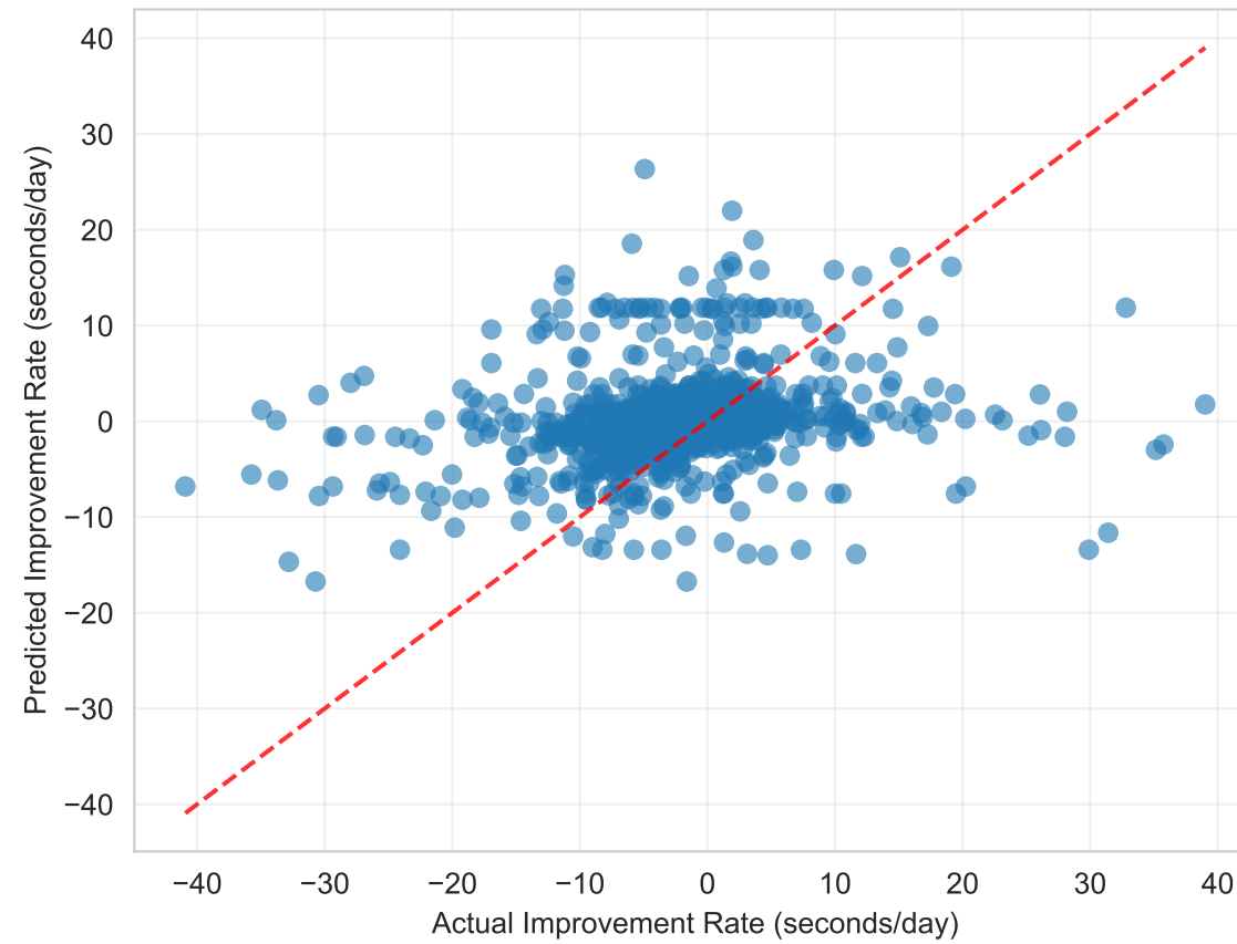
Gradient Boosting R^2 = -0.1394
