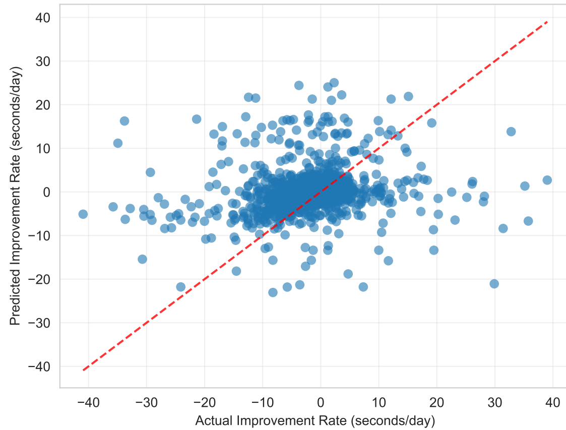
Random Forest R^2 = -0.3247
