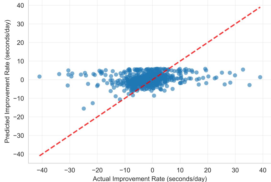
Random Forest R^2 = -0.368 (95% CI: [-0.577, -0.205]) n=1164
