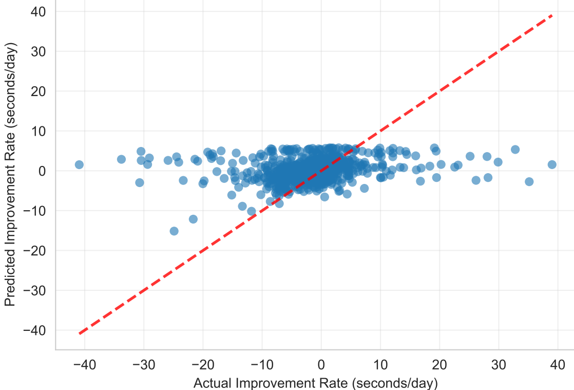
Gradient Boosting R^2 = -0.160 (95% CI: [-0.324, -0.033]) n=1164
