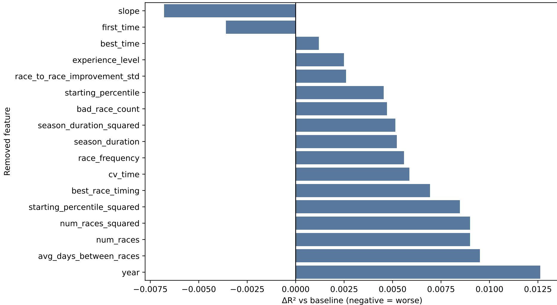
Feature ablation: \Delta R^2 after removing one feature (F only) (Train 2023 \rightarrow Test 2024, Random Forest)
