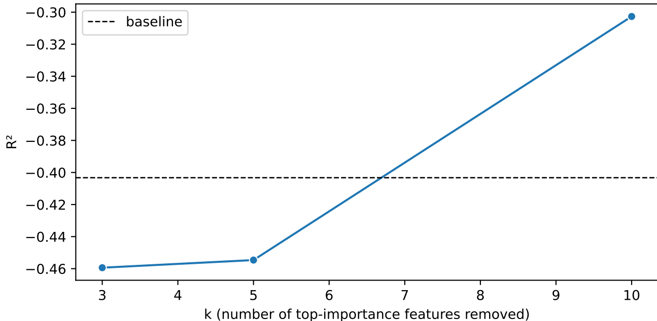
Drop top-k important features: R^2 (M only) (Train 2023 \rightarrow Test 2024, Random Forest)
