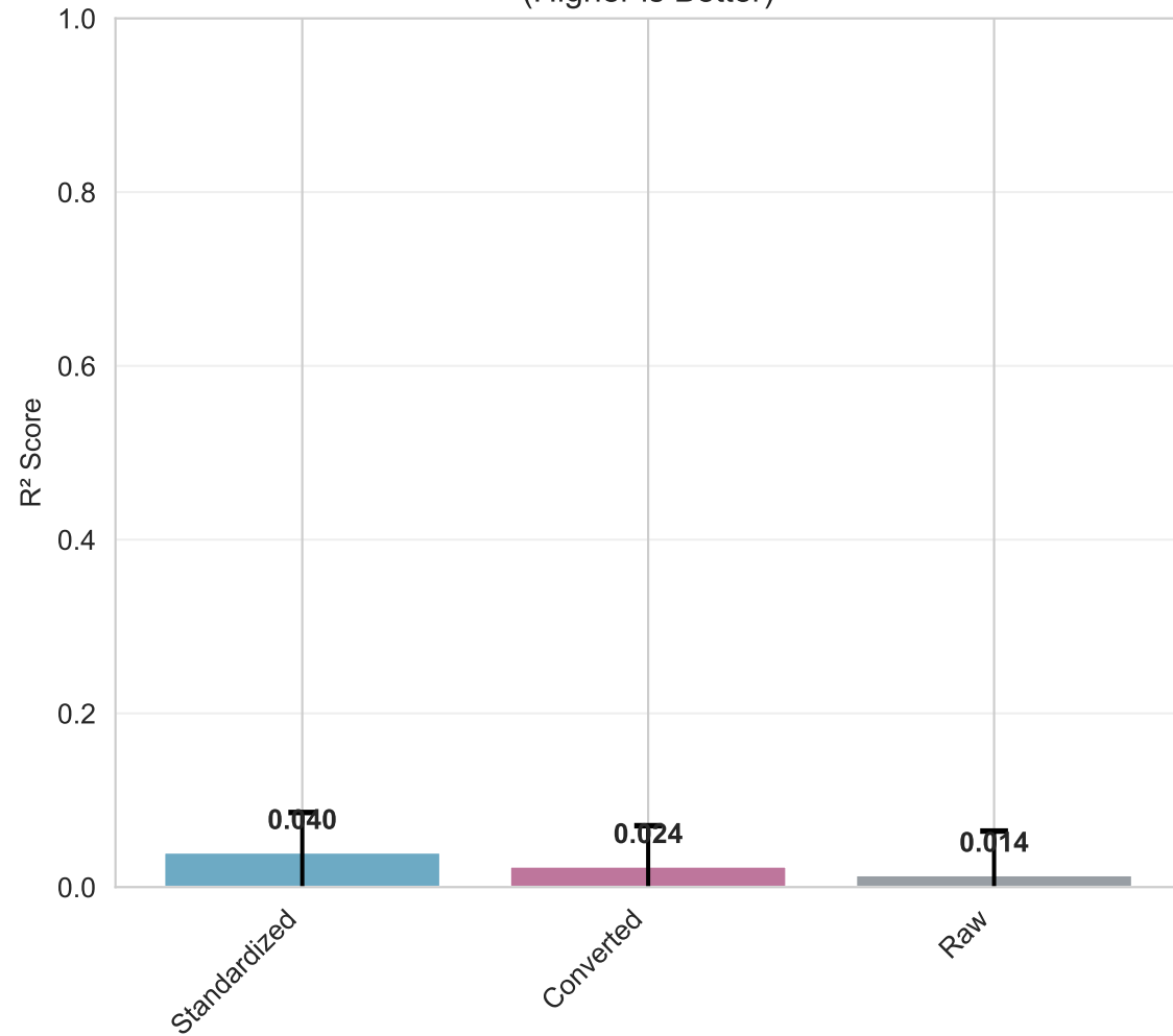
Model Performance by Time Standardization Method (SVR - Same Model for All Methods) (Higher is Better)
