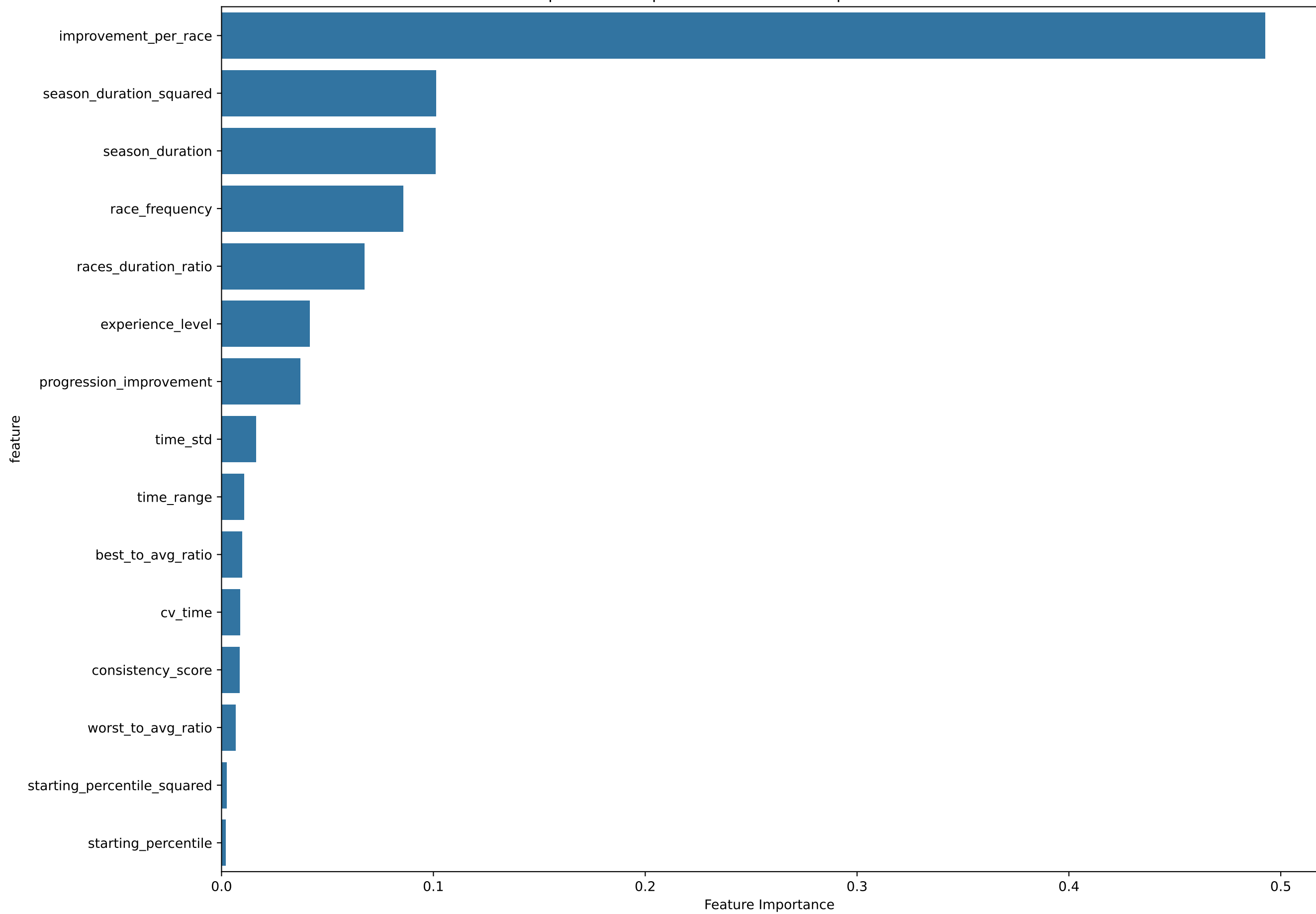
Top 15 Most Important Features for Improvement Prediction
