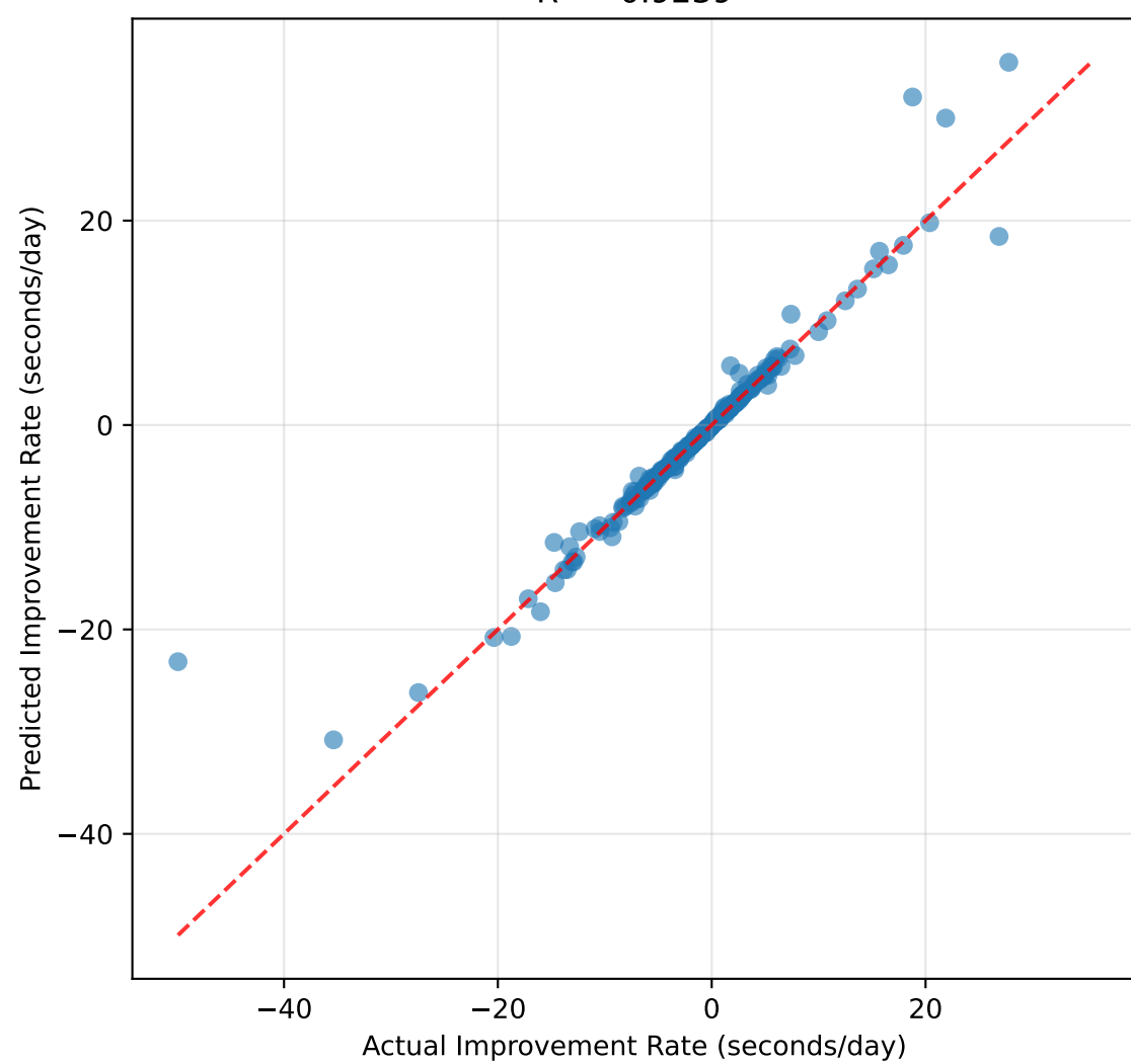
Random Forest R^2 = 0.9239
