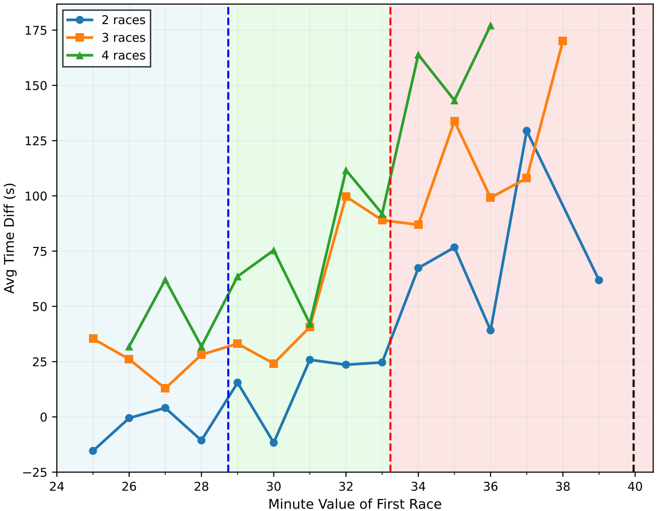
2024: Converted Only (distance) - Male IQR: Q1=28min, Q3=33min
