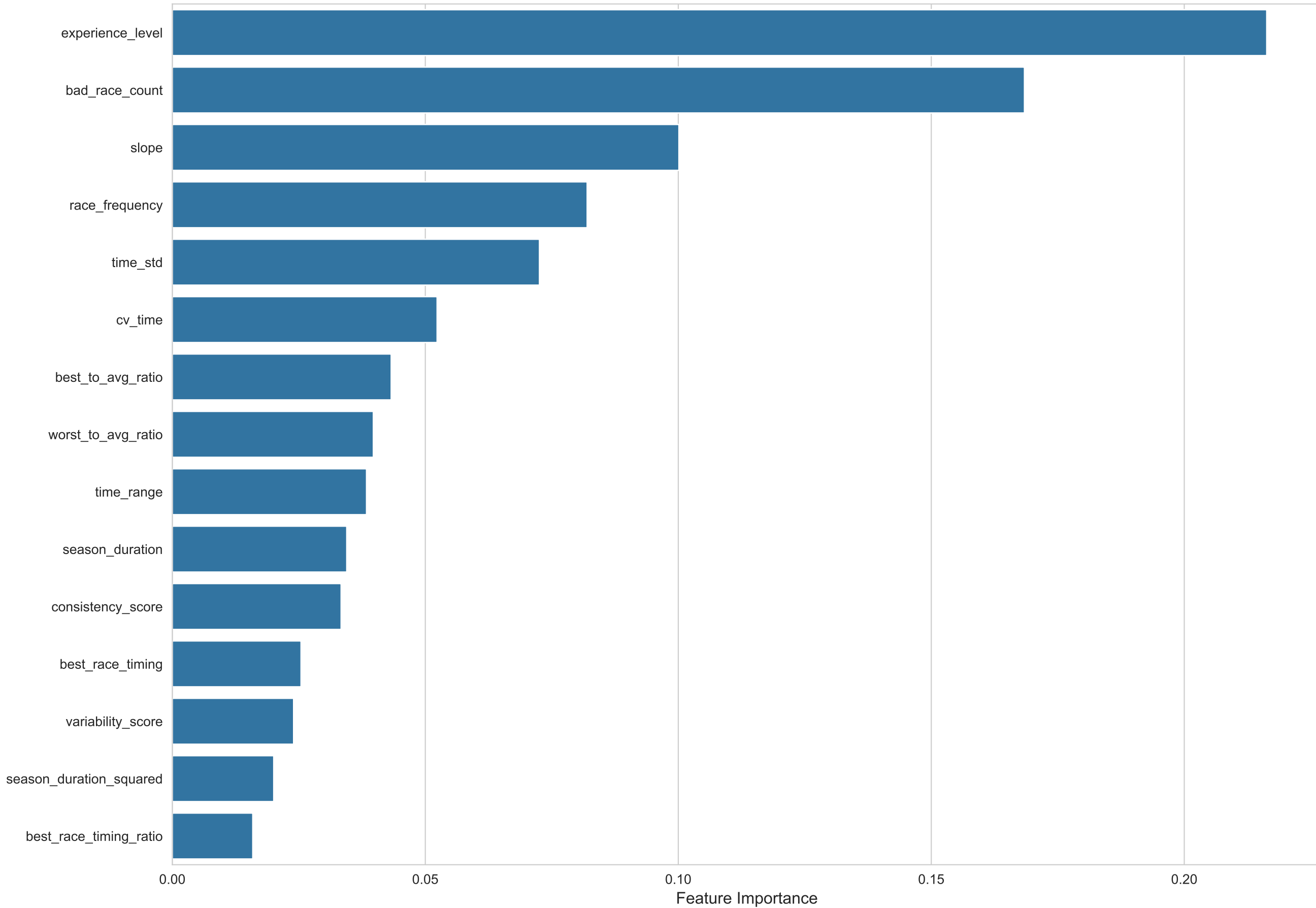
Top 15 Most Important Features for Improvement Prediction Random Forest Feature Importance
