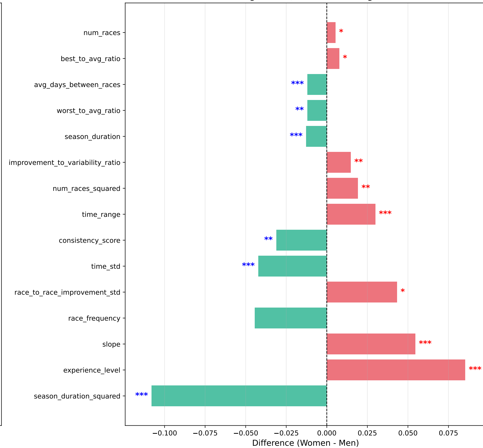
Feature Importance Differences (Red/Green = FDR Significant, Gray = Not Significant) FDR: 15 significant, Bonferroni: 7 significant
